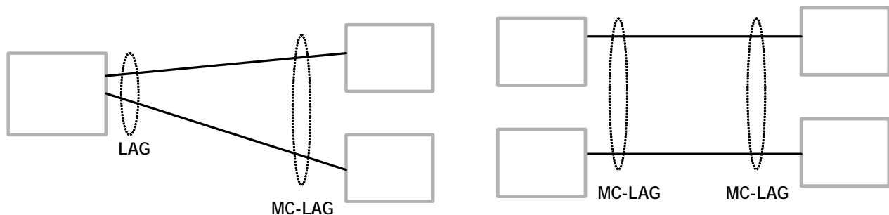
Figure 6: Active-Standby LAG Operation without LACP
