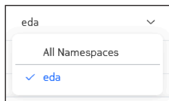
Figure 30: Namespace selector
