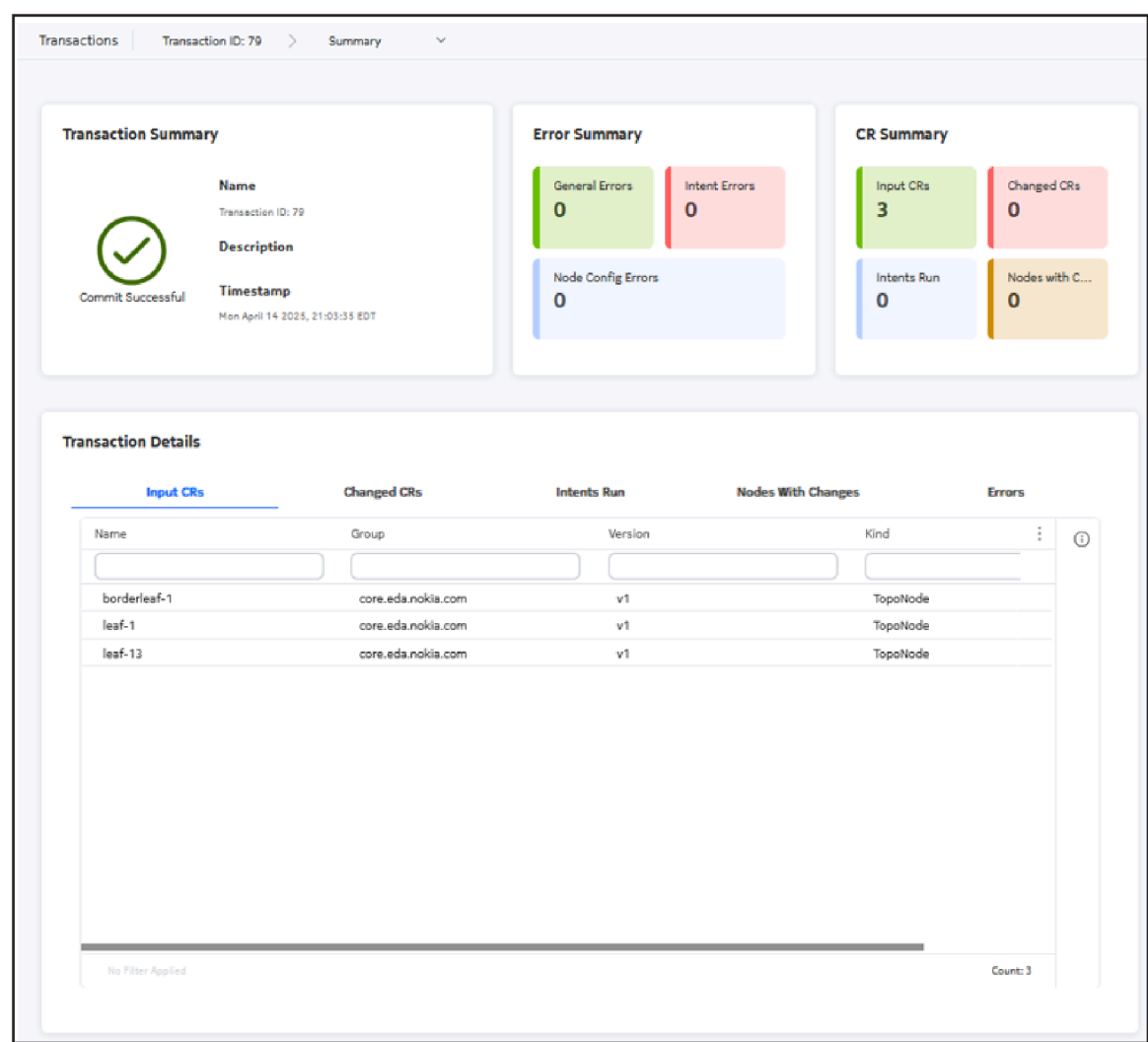
Figure 54: The Transactions summary page
