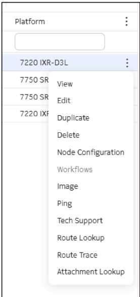
Figure 58: Row actions
