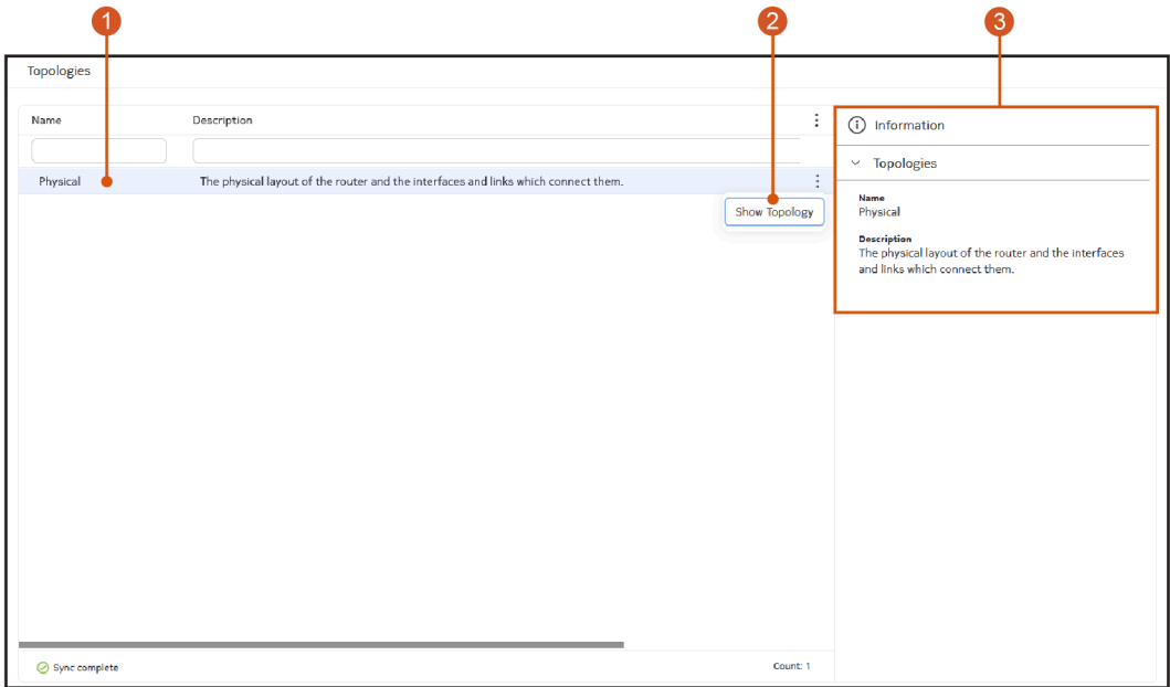
Figure 61: The Topologies page
