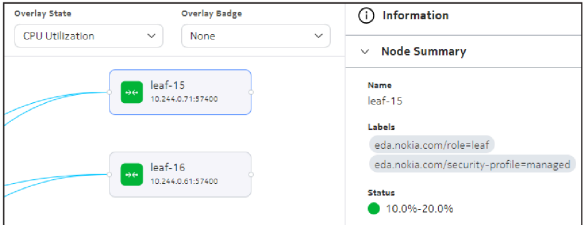
Figure 63: CPU Utilization Overlay and information panel
