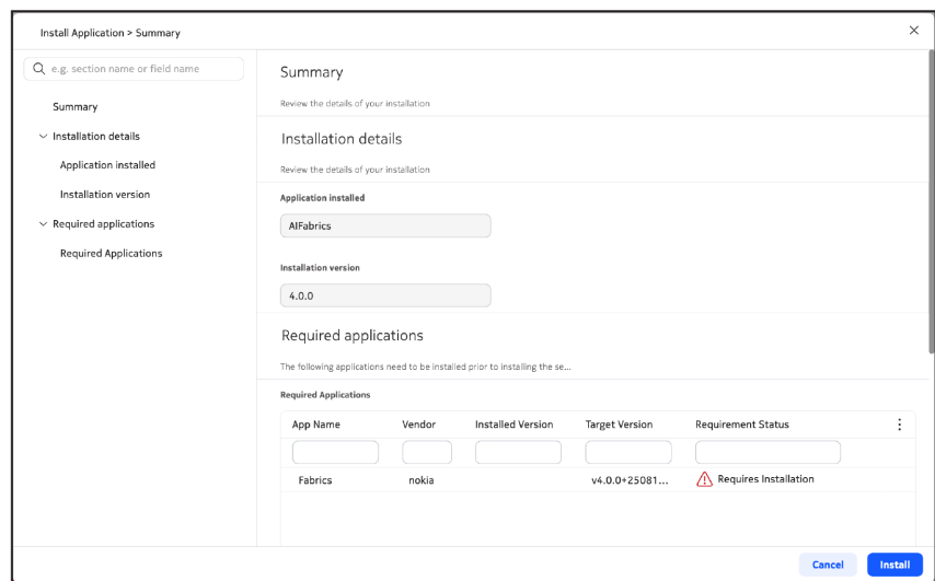
Figure 73: Summary page for an app with requirements
