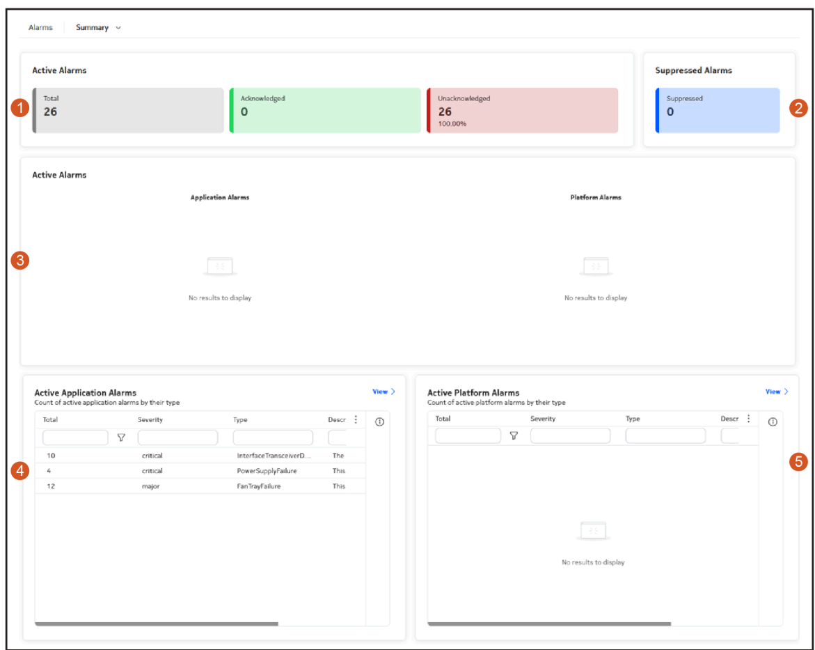
Figure 41: The Alarms Summary page
