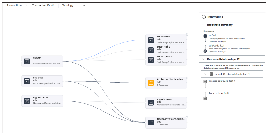
Figure 56: The Transactions Topology view
