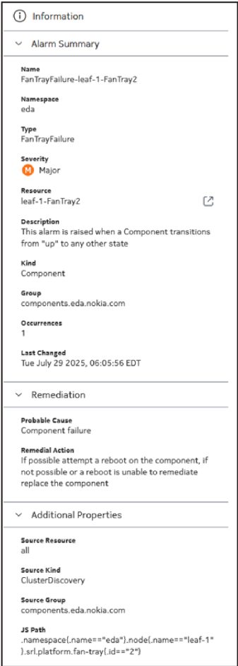
Figure 43: The expanded Alarms Information panel
