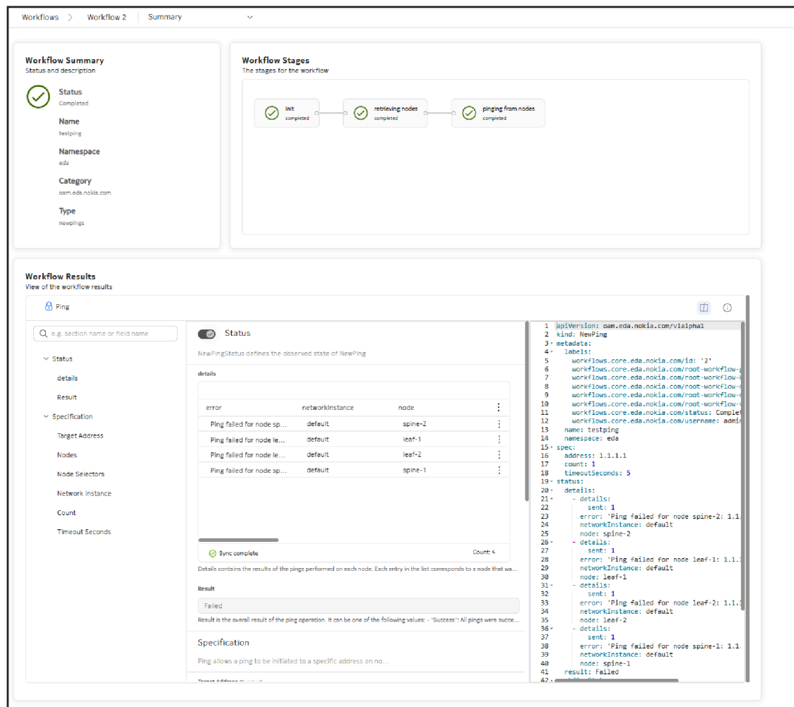
Figure 38: Workflow Summary page
