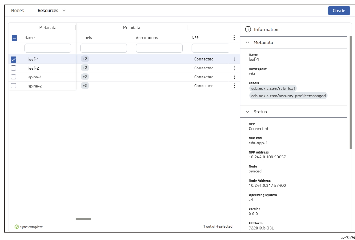
Figure 7: An example of an expanded information panel, showing the collapse control
