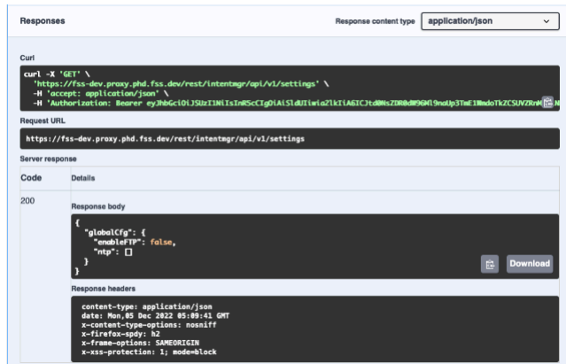
Figure 5: Responses section
