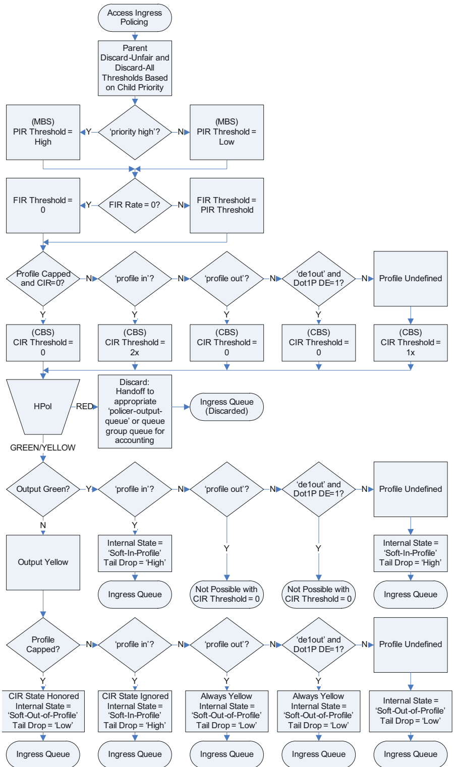
Figure 25: Ingress Policer Threshold Determination and Output Behavior
