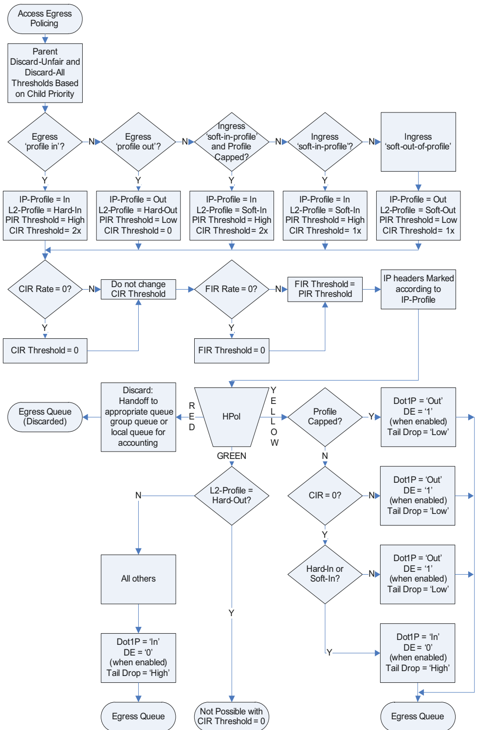
Figure 26: Egress Policer Threshold Determination and Output Behavior
