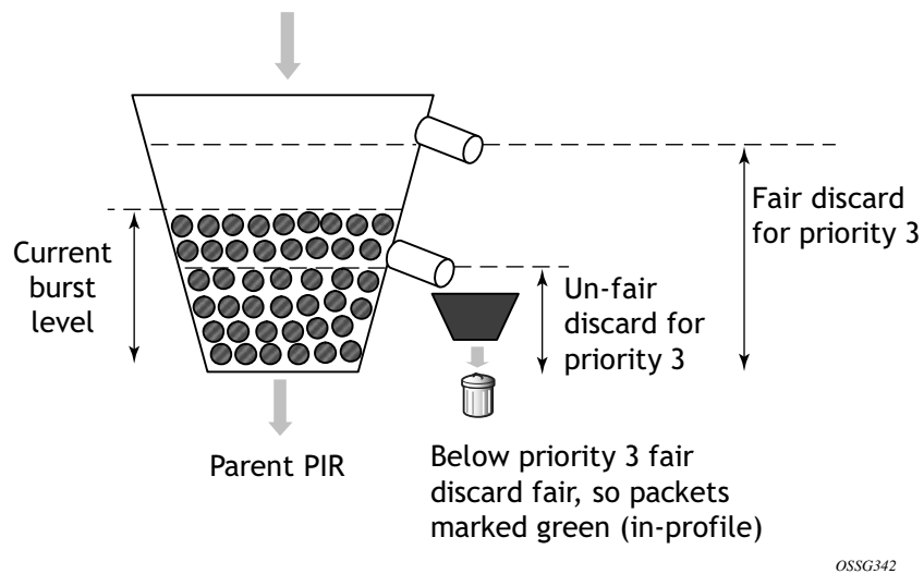
Figure 24: Parent Policer Bucket and Priority Thresholds
