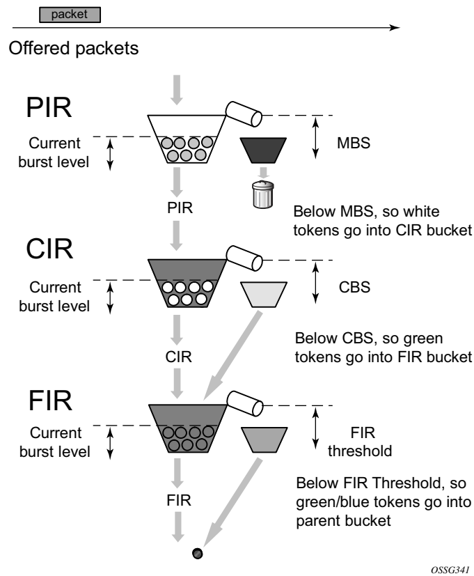
Figure 23: Policer Bucket Rate and Packet Flow Interaction with Bucket Depth
