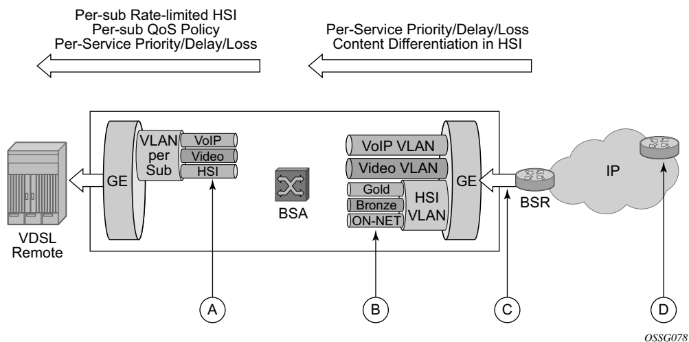
Figure 3: Downstream QoS Enablement
