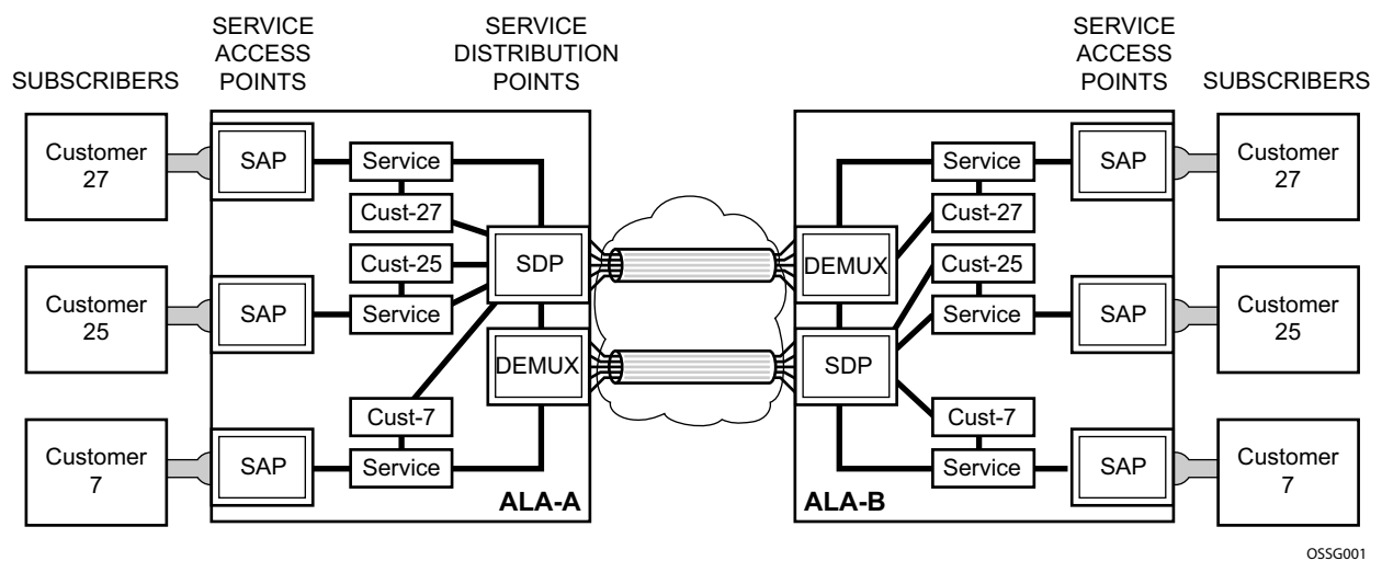
Figure 8: Alcatel-Lucent's Service Entities
