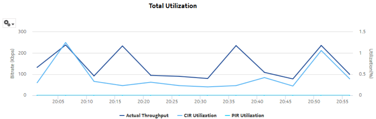
Figure 14-11 SAP Utilization Details report—Ingress utilization
