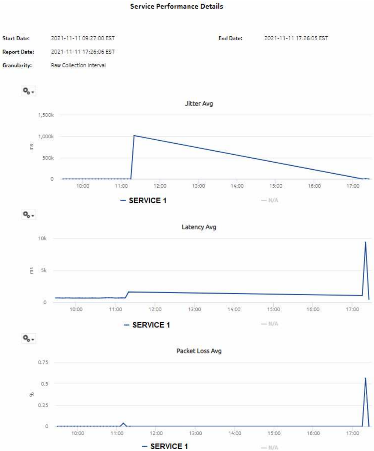
Figure 11-16 Service Performance Details report
