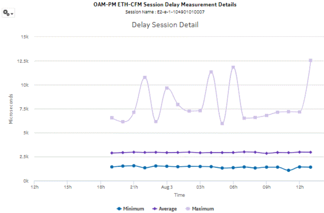
Figure 13-8 OAM-PM ETH-CFM Session Delay Measurement Details report
