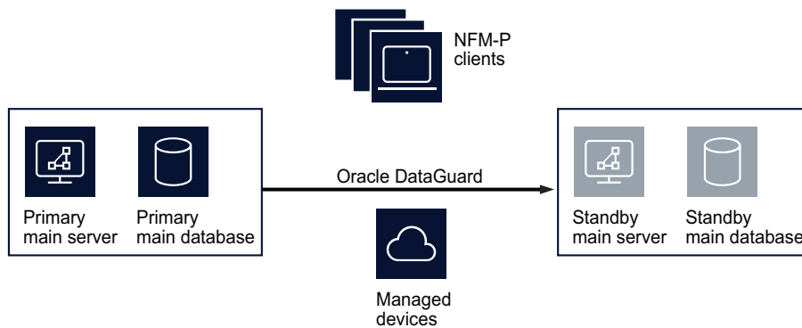
Figure 17-1 Collocated redundant NFM-P deployment
