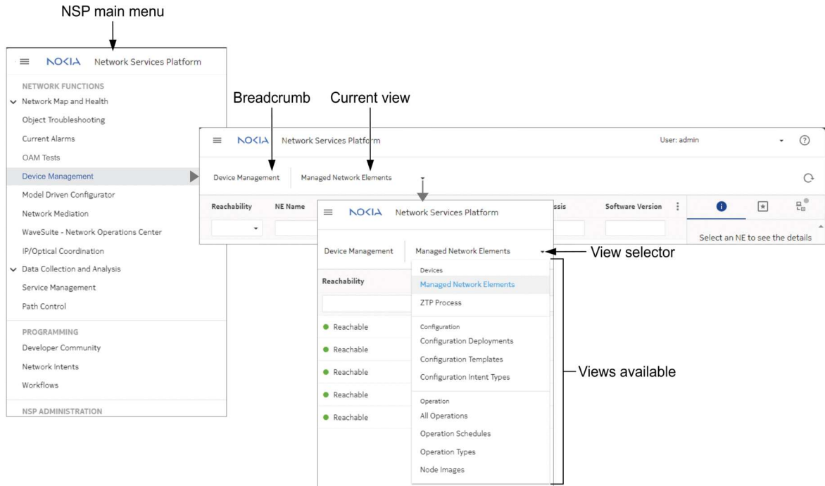
Figure 1-3 Navigation flow
