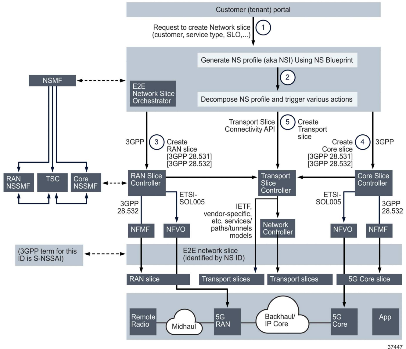
Figure 1-2 Network slice creation
