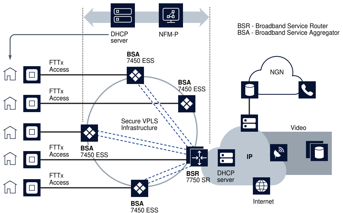
Figure 70-13 TPSDA components
