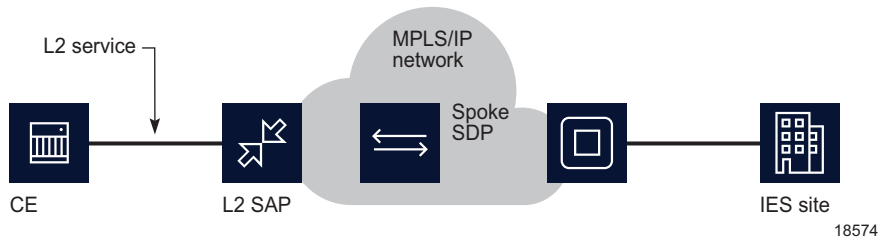
Figure 78-2 SDP spoke termination on an L2 service
