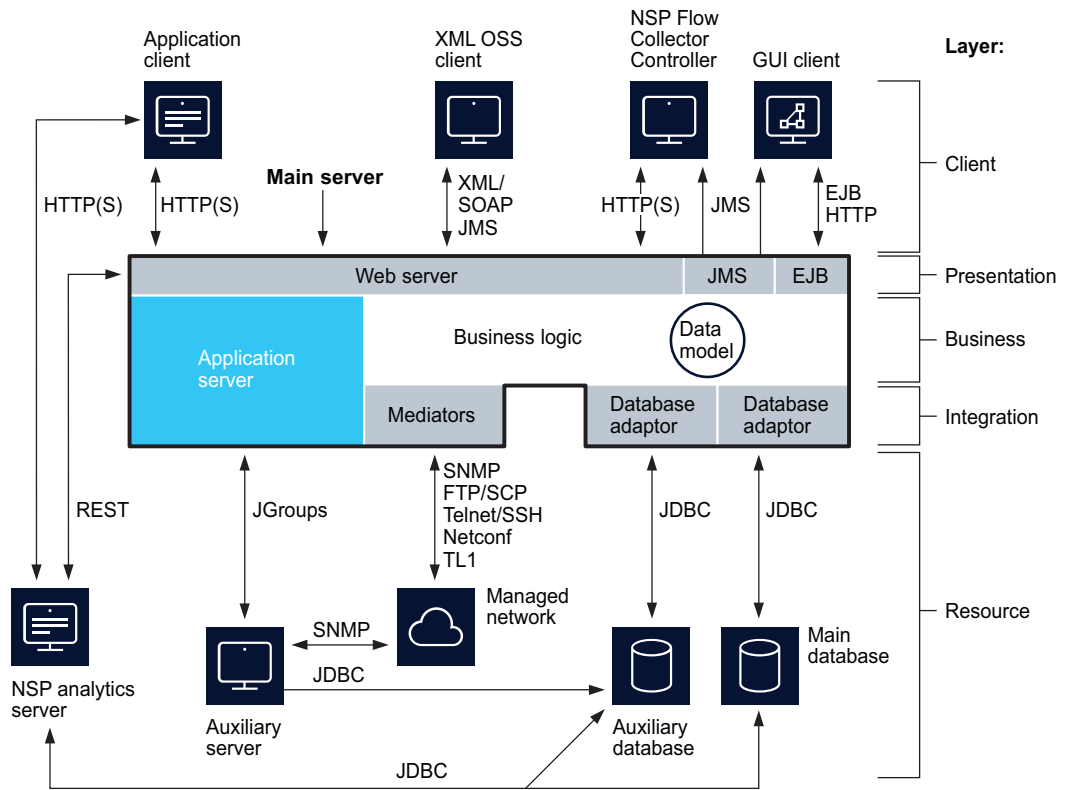
Figure 3-2 NFM-P multi-layer model
