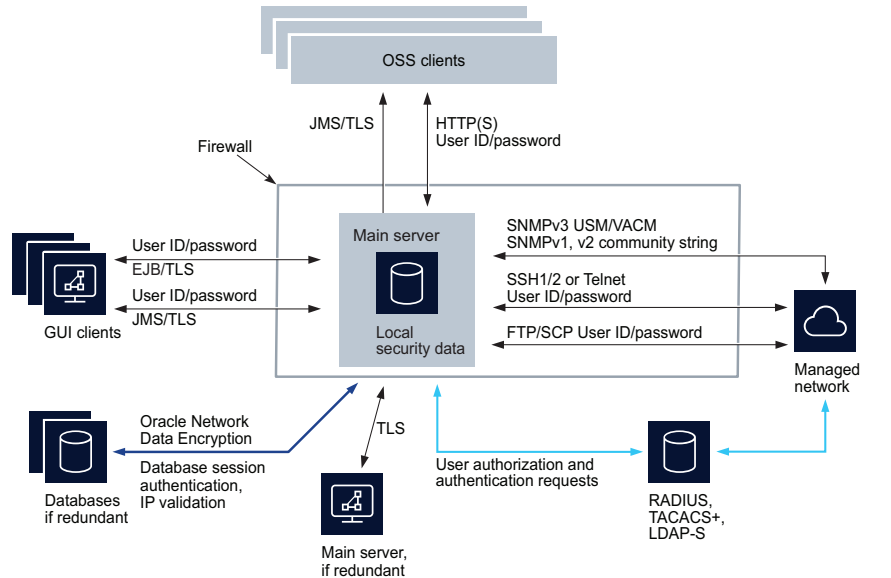
Figure 6-2 NFM-P security mechanisms
