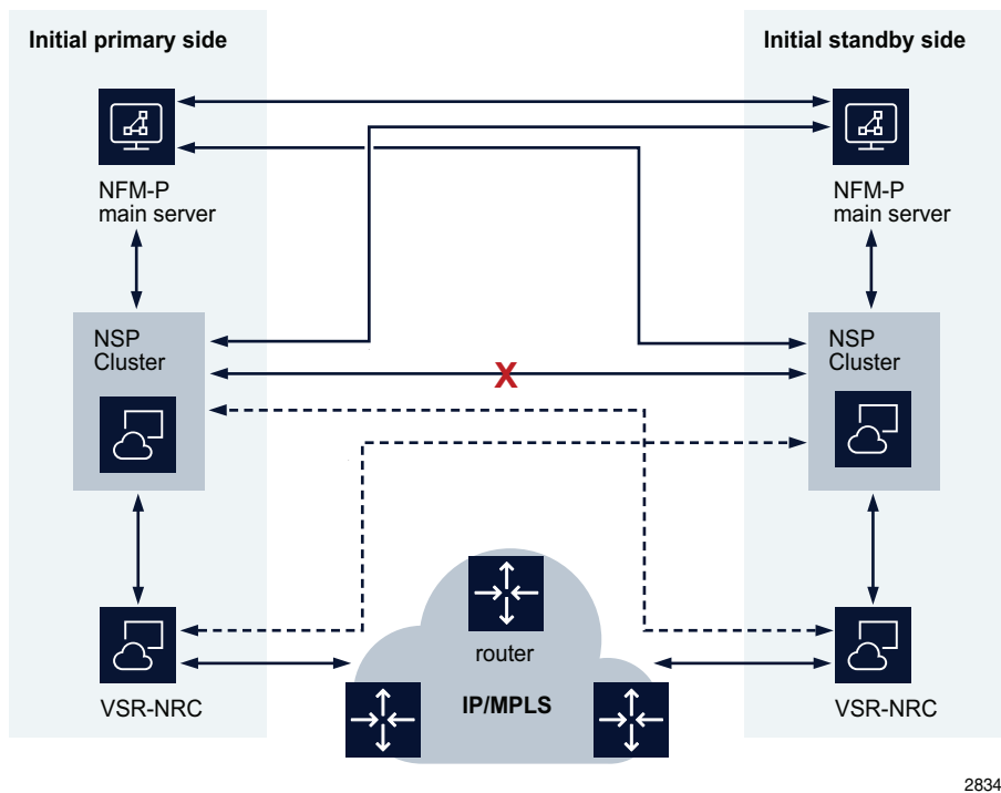
Figure 8-2 Primary and standby NSP cluster communication failure
