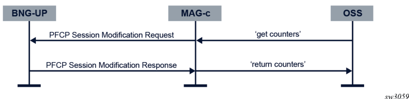
Figure 8: MAG-c triggered accounting update
