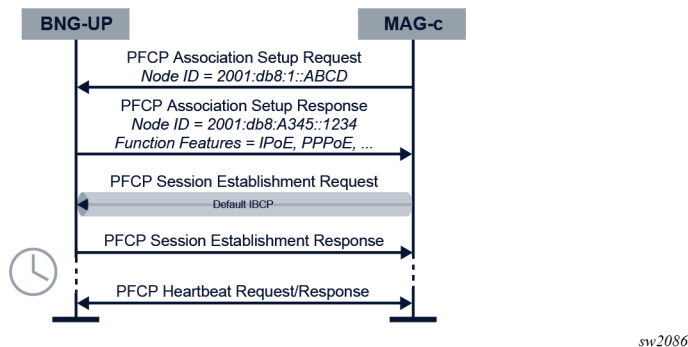
Figure 5: Initial PFCP association and session setup
