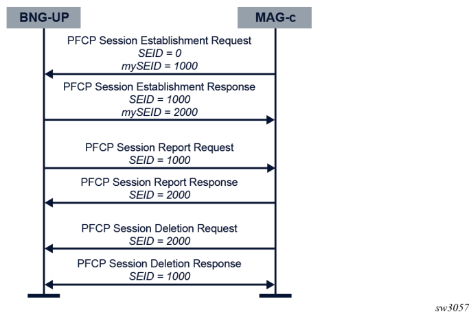
Figure 4: PFCP session ID allocation and use
