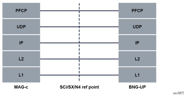
Figure 3: PFCP protocol stack for the control plane
