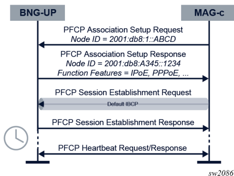
Figure 5: Initial PFPC association and session setup
