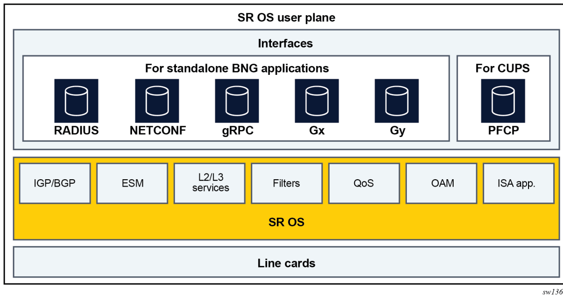
Figure 4: MAG-u interfaces and key applications
