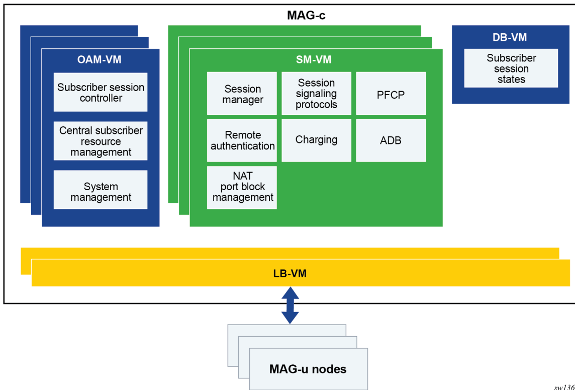
Figure 3: MAG-c functional blocks and VNF grouping
