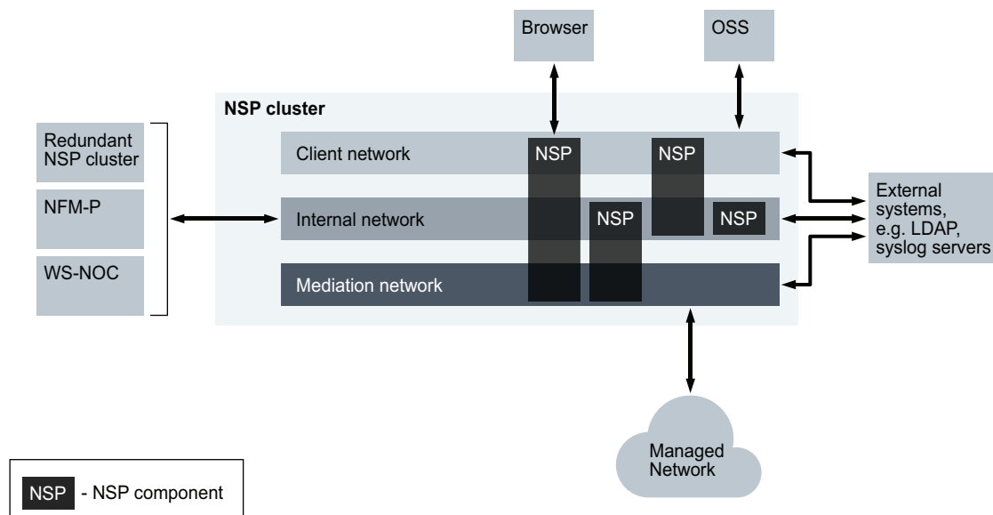
Figure 7-1 NSP multi-interface communication
