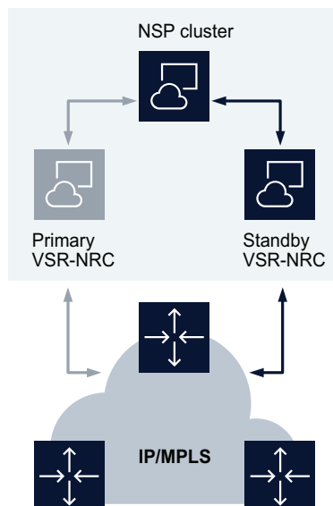
Figure 8-4 Primary VSR-NRC failure in single-site deployment
