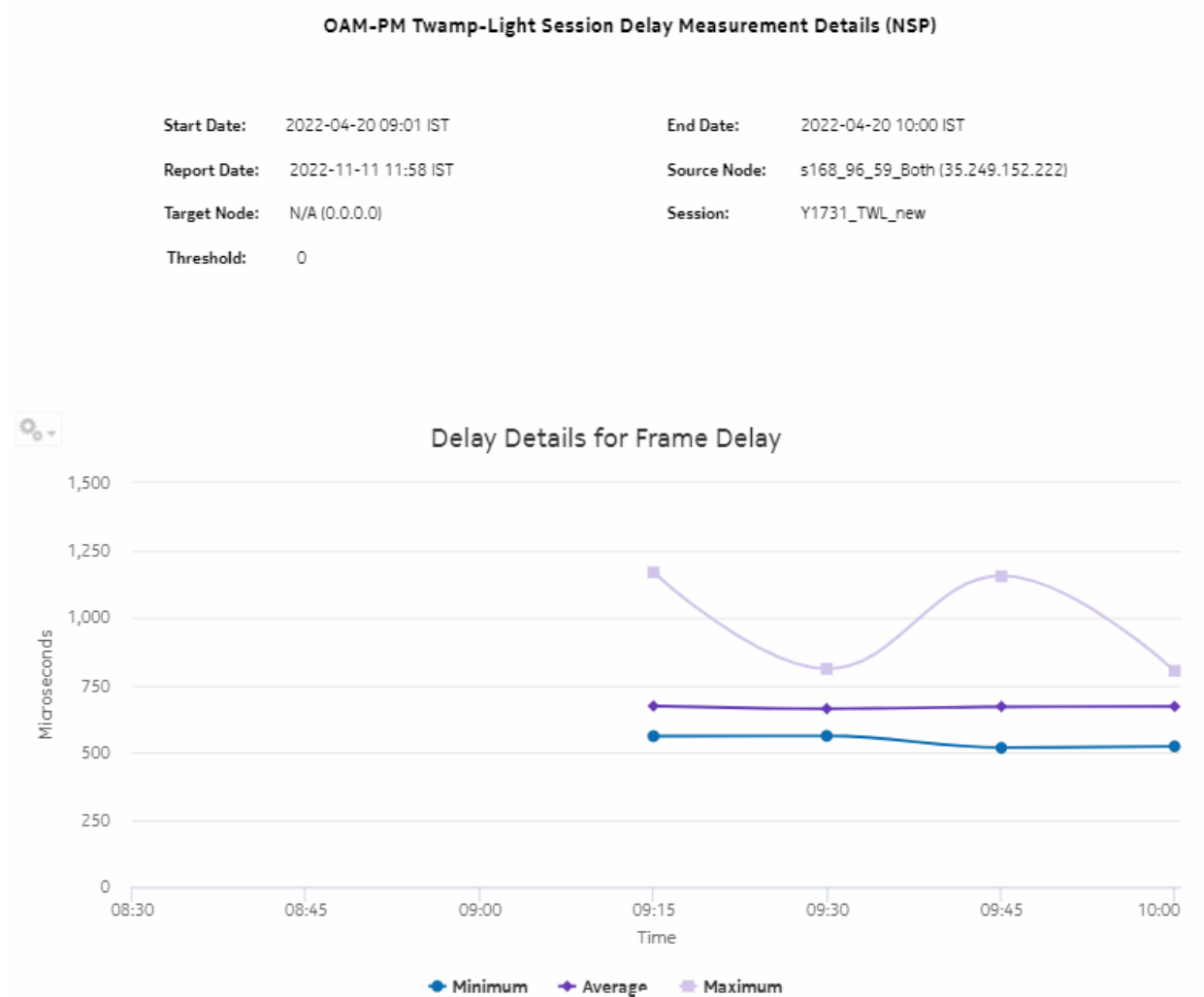
Figure 17-7 OAM-PM Twamp-Light Session Delay Measurement Details (NSP) – Delay Details for Frame Delay
