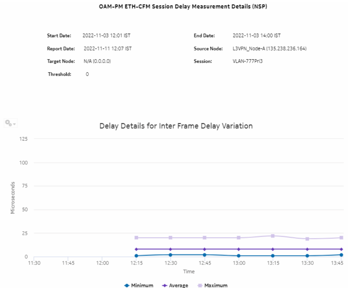
Figure 17-11 OAM-PM ETH-CFM Session Delay Measurement Details (NSP) – Delay Details for Inter Frame Delay Variation
