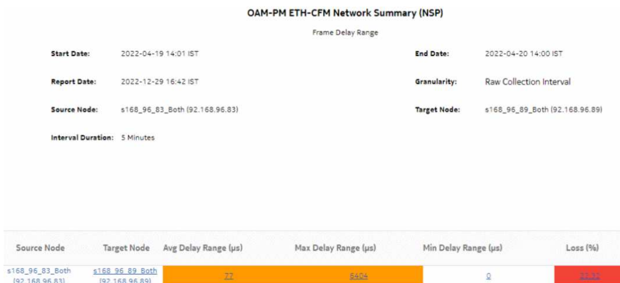
Figure 17-23 OAM-PM ETH-CFM Network Summary (NSP) – Frame Delay Range
