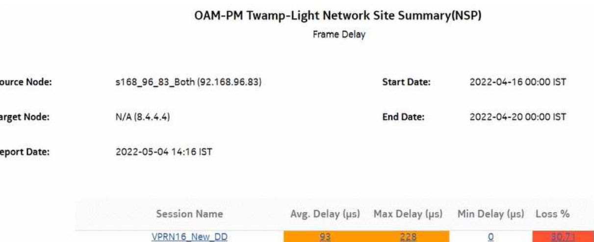
Figure 17-17 OAM-PM Twamp-Light Network Site Summary (NSP) – Frame Delay
