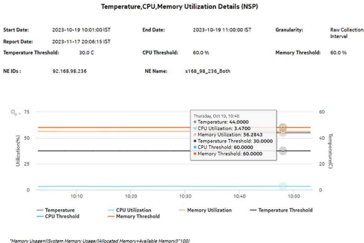
Figure 18-14 Temperature, CPU, Memory Utilization Details (NSP) report
