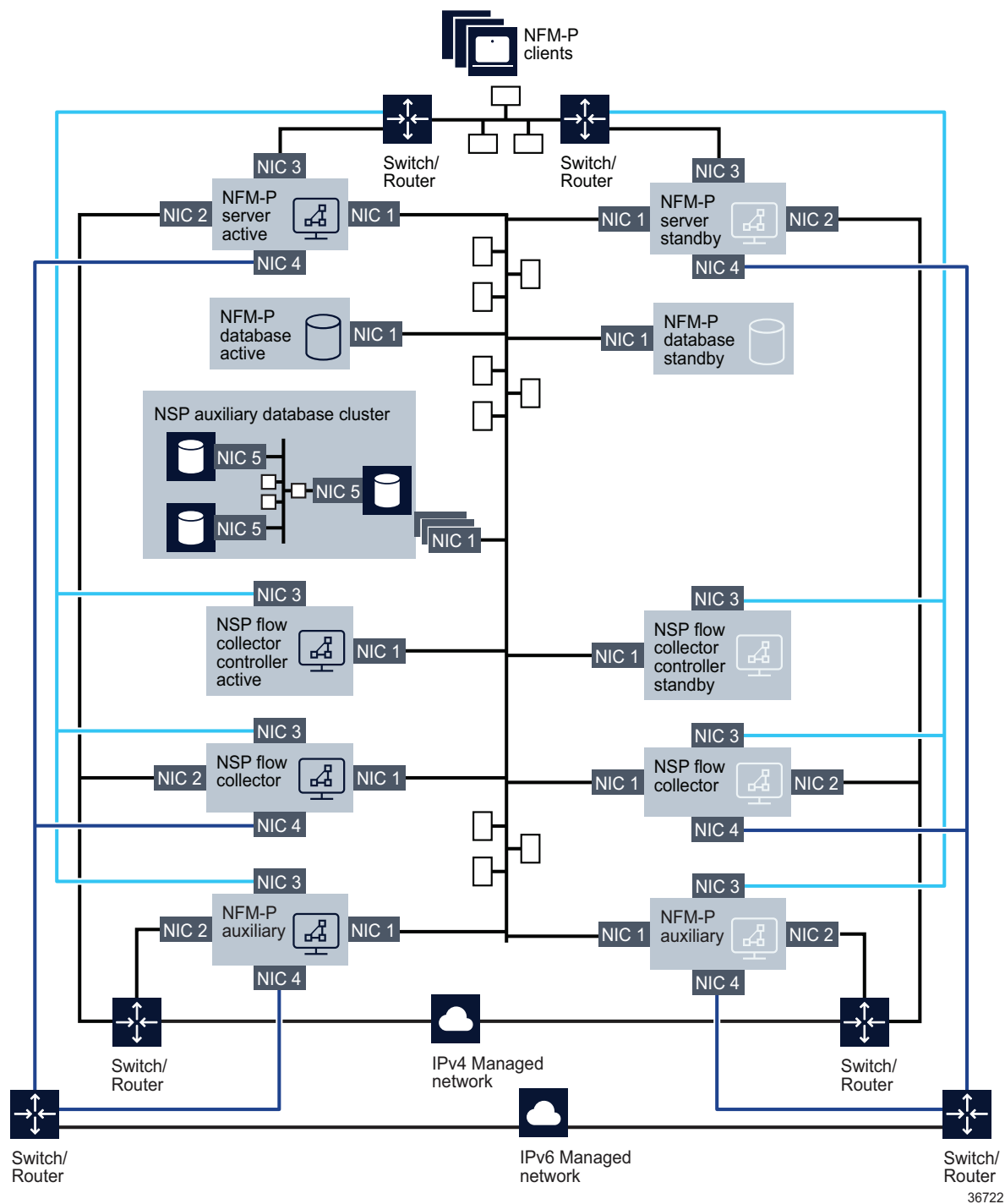
Figure 7-3 Distributed NFM-P server/database deployment with multiple network interfaces
