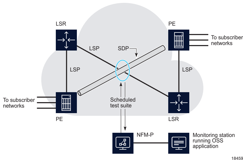
Figure 89-1 Sample STM implementation
