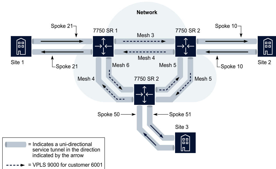
Figure 77-1 HVPLS configuration
