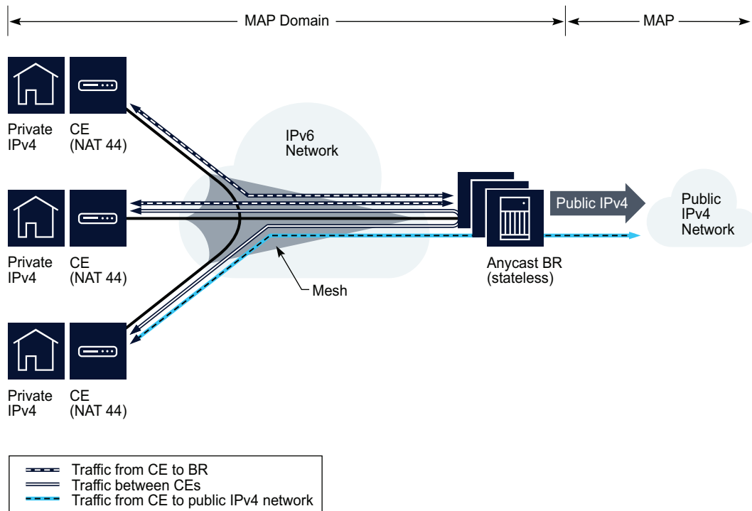
Figure 64-1 MAP-T domain
