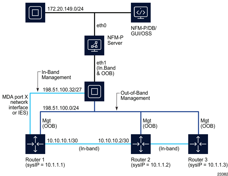
Figure 8-1 Example of in-band and out-of-band management
