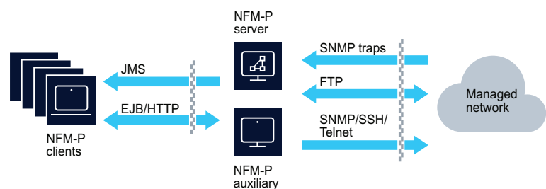
Figure 6-2 Firewalls and NFM-P standalone deployments
