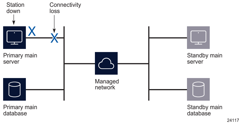
Figure 17-12 Primary server unreachable, distributed system
