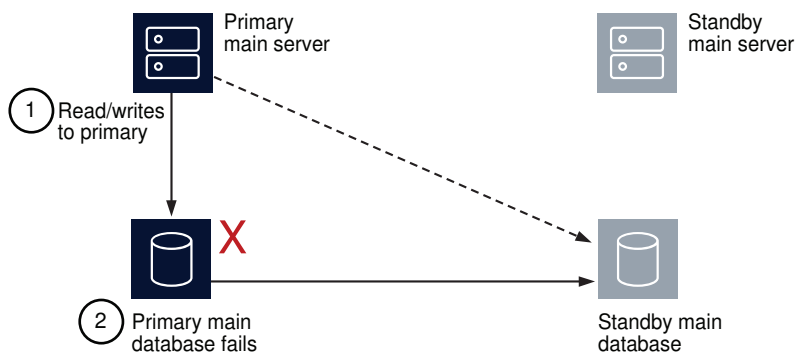
Figure 17-8 Server and database roles before database failover
