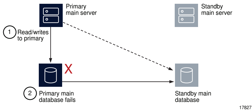
Figure 17-8 Server and database roles before database failover
