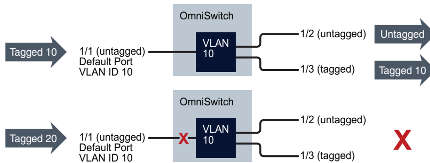
Figure 16-2 Tagged traffic and VLANs
