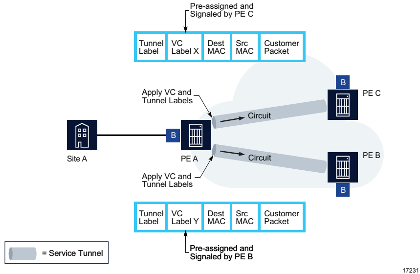
Figure 77-14 Packet forwarding from PE A across the core IP/MPLS network
