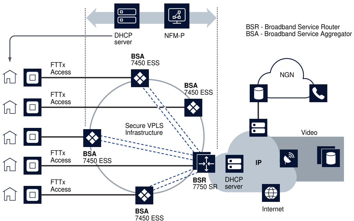
Figure 70-13 TPSDA components
