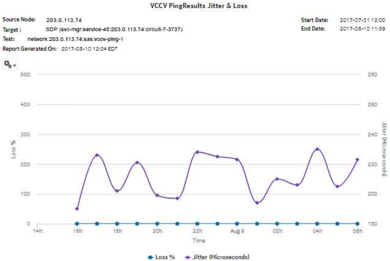
Figure 13-34 VCCV Ping Results Jitter & Loss report
