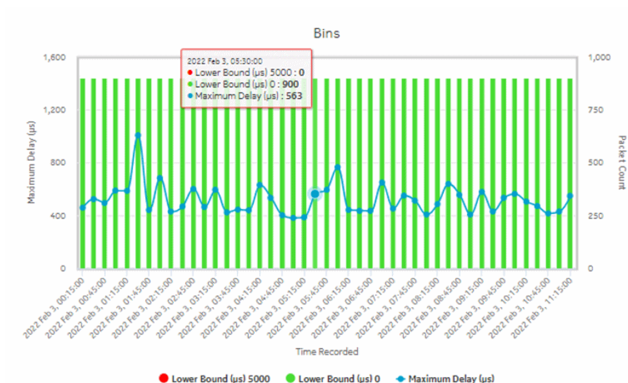
Figure 18-4 OAM-PM Bins and Delay report – NFM-P NE CFM DMM session bins and delay
