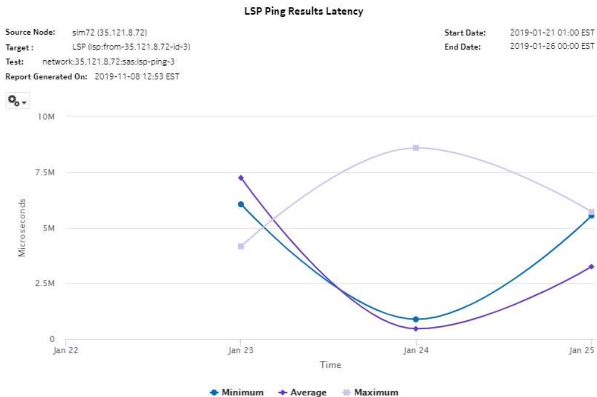
Figure 13-30 LSP Ping Results Latency report
