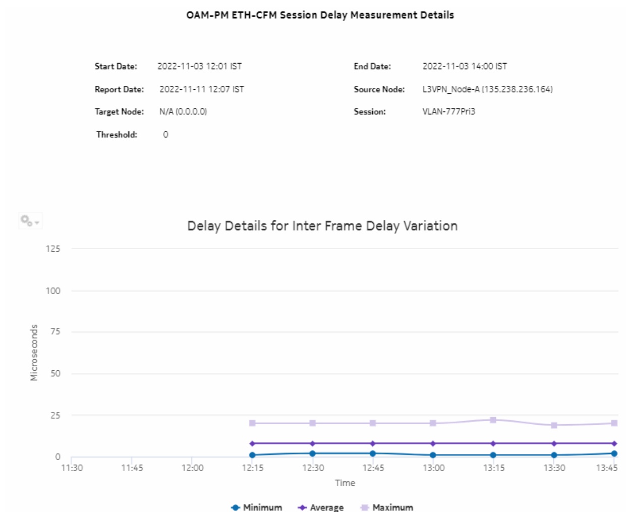
Figure 18-11 OAM-PM ETH-CFM Session Delay Measurement Details – Delay Details for Inter Frame Delay Variation
