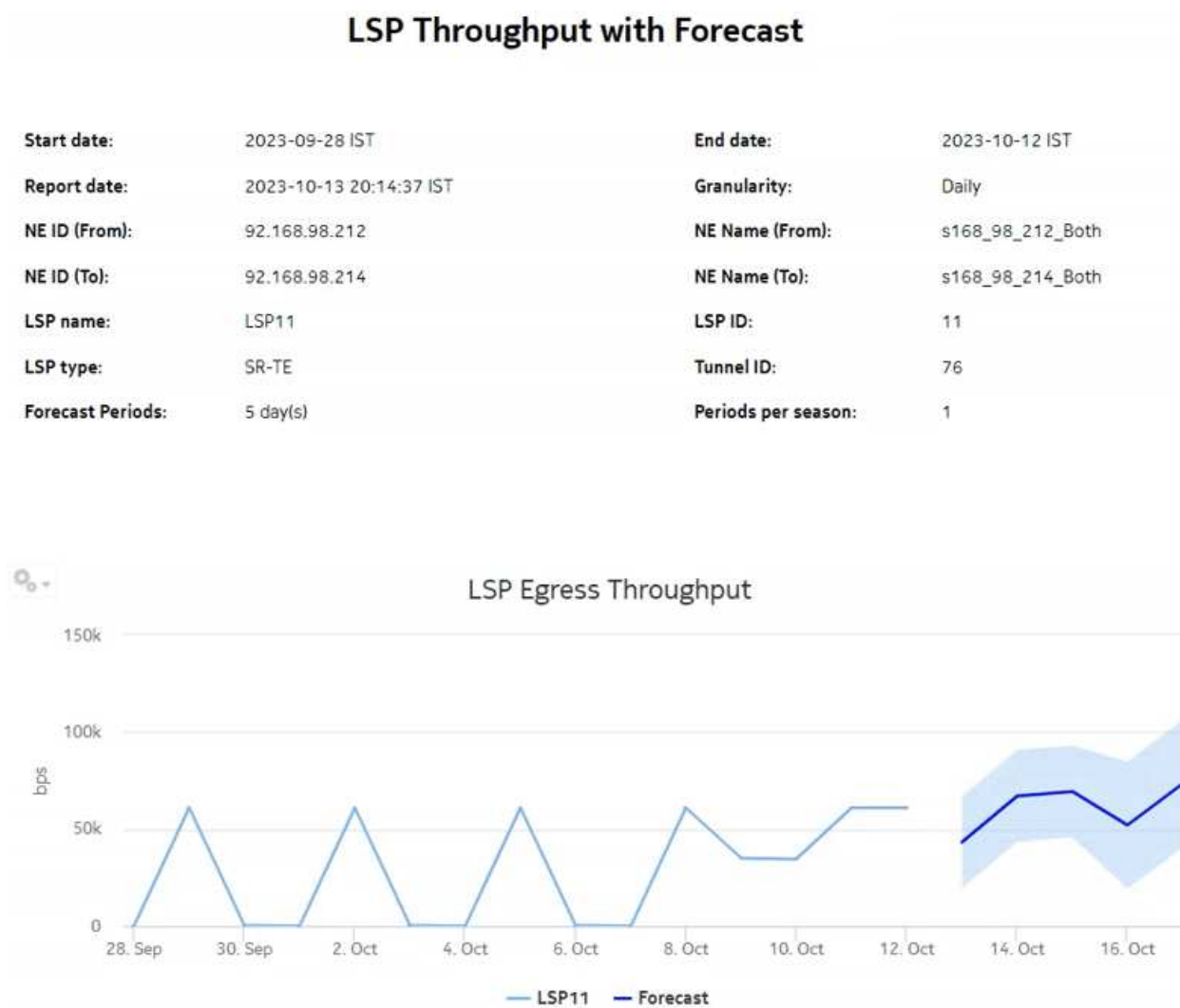
Figure 19-4 LSP Throughput with Forecast report—For LSPs managed by the 7750 MD SR
