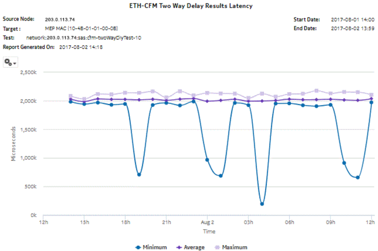
Figure 13-27 ETH-CFM Two Way Delay Results Latency report
