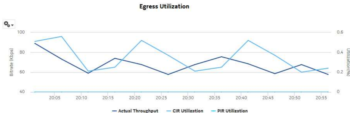
Figure 14-8 SAP Utilization Details report—Egress utilization
