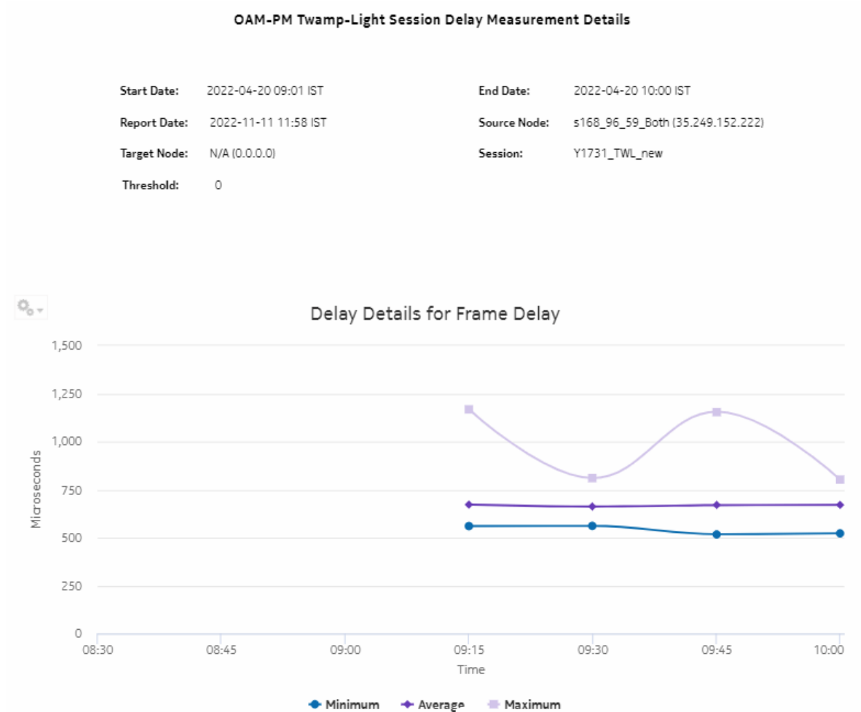
Figure 18-7 OAM-PM Twamp-Light Session Delay Measurement Details – Delay Details for Frame Delay
