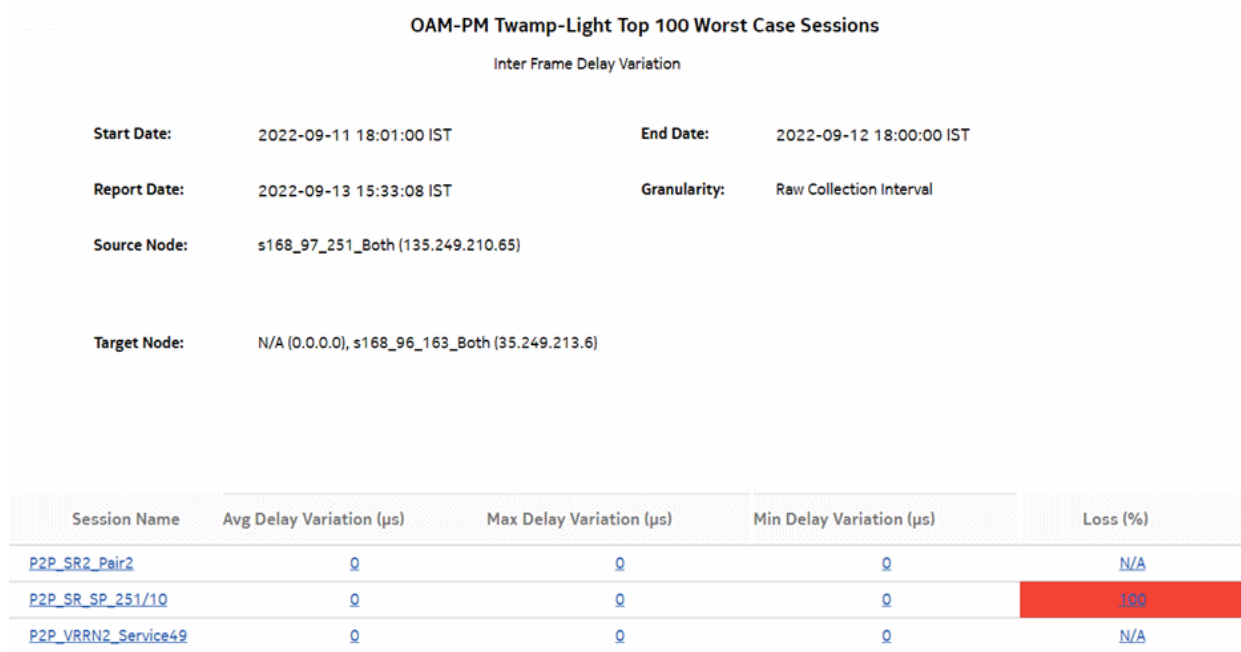
Figure 18-41 OAM-PM Top N Worst Sessions—Inter Frame Delay Variation
