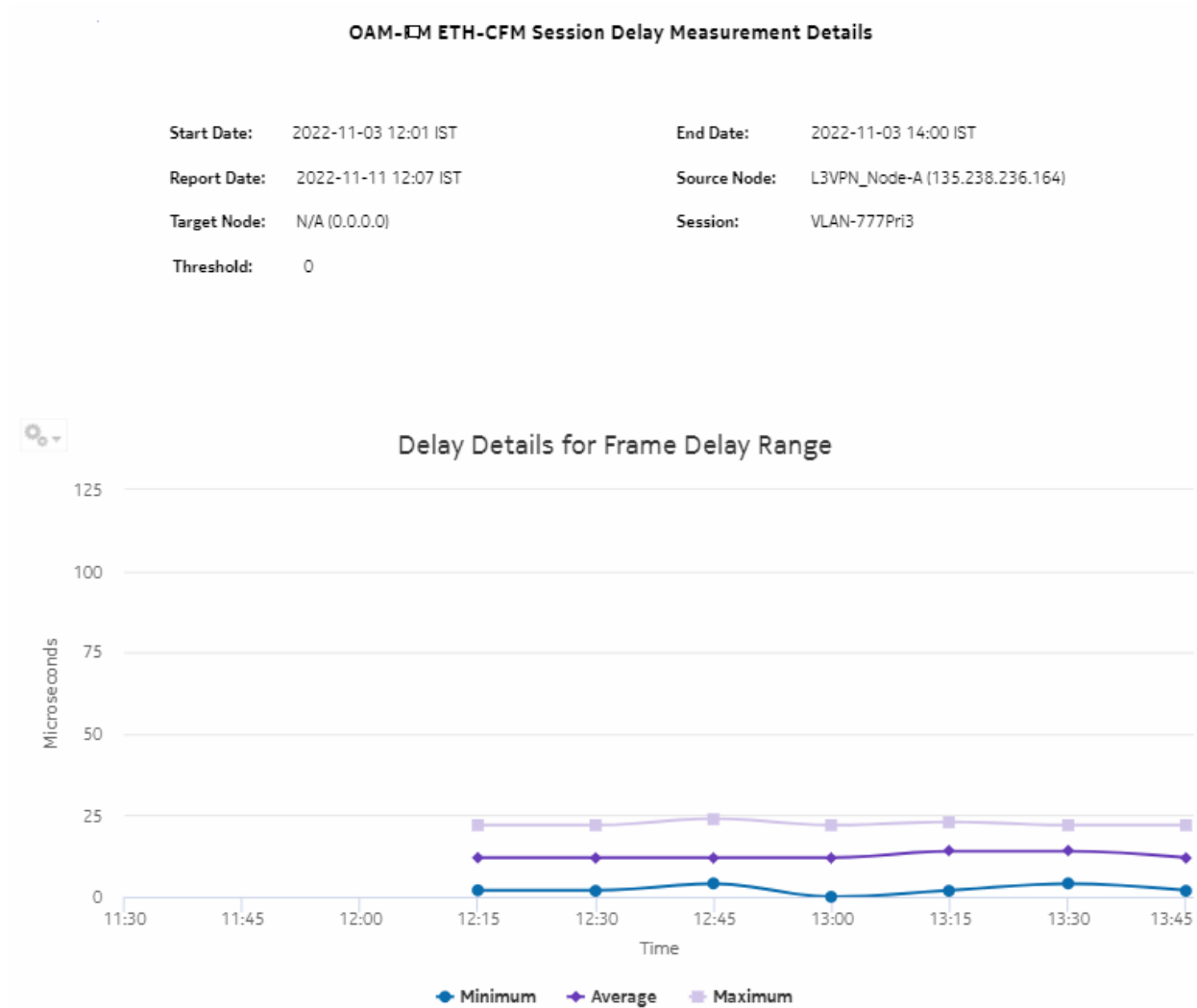
Figure 18-9 OAM-PM ETH-CFM Session Delay Measurement Details – Delay Details for Frame Delay Range
