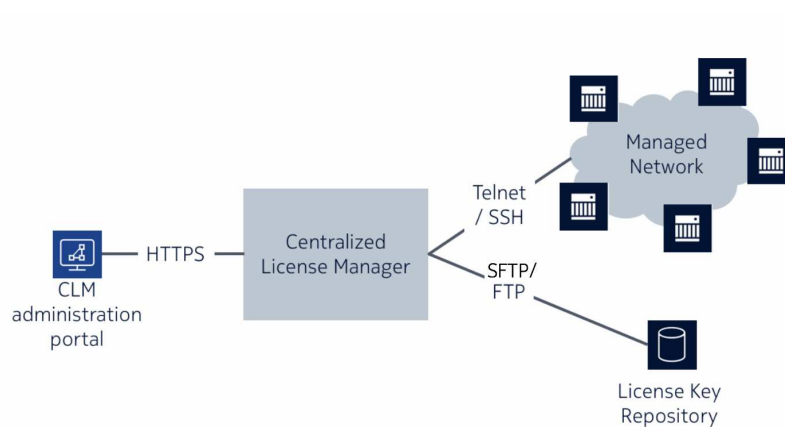
Figure 1-1 CLM architecture
