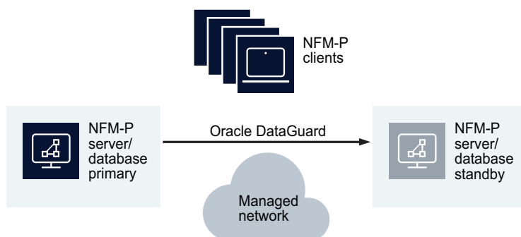
Figure 1-8 NFM-P collocated server/database redundancy deployment
