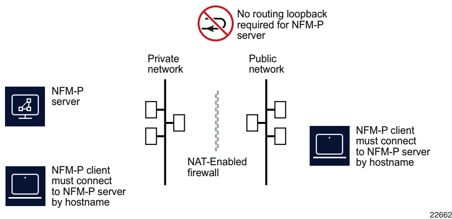
Figure 7-5 NFM-P server deployment using NAT with name resolution based communication
