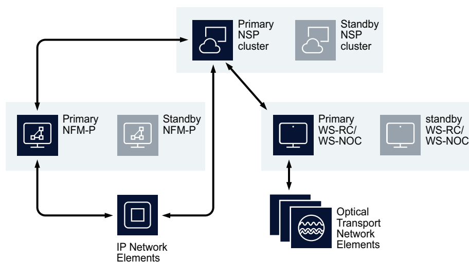
Figure 1-3 DR NSP deployment including NFM-P and WS-NOC
