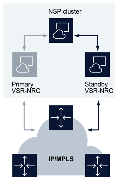
Figure 8-3 Primary VSR-NRC failure in single-site deployment
