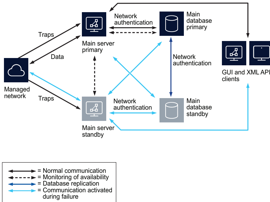
Figure 8-2 Redundant NFM-P system
