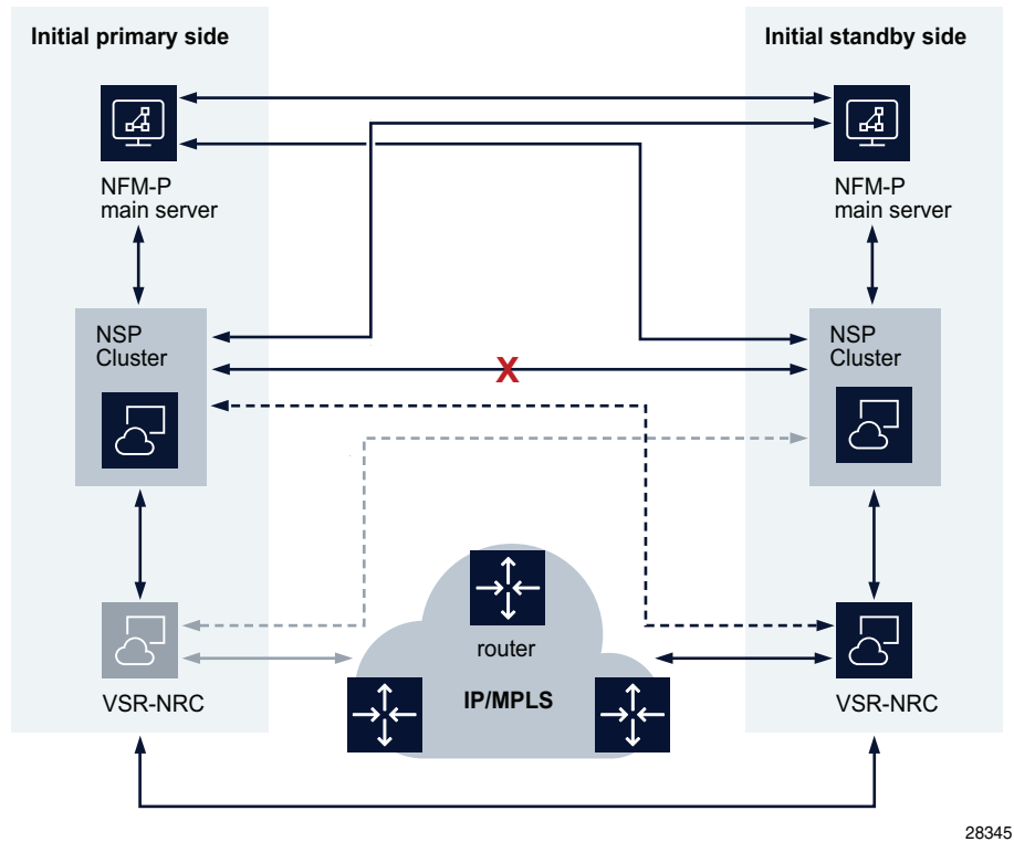
Figure 8-4 Primary VSR-NRC failure in a dual-site deployment
