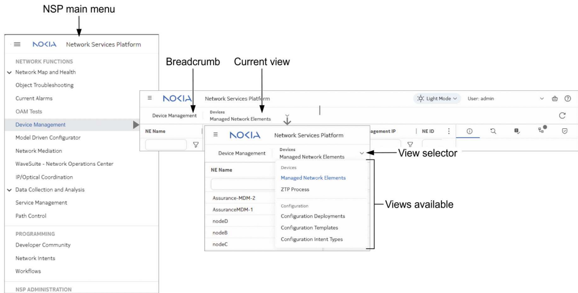
Figure 2-2 Navigation flow
