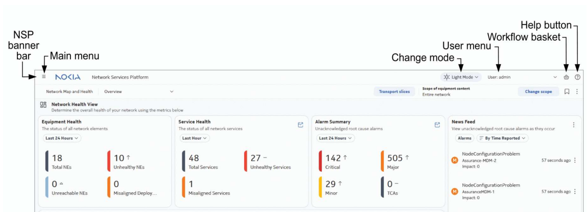
Figure 2-1 Banner bar
