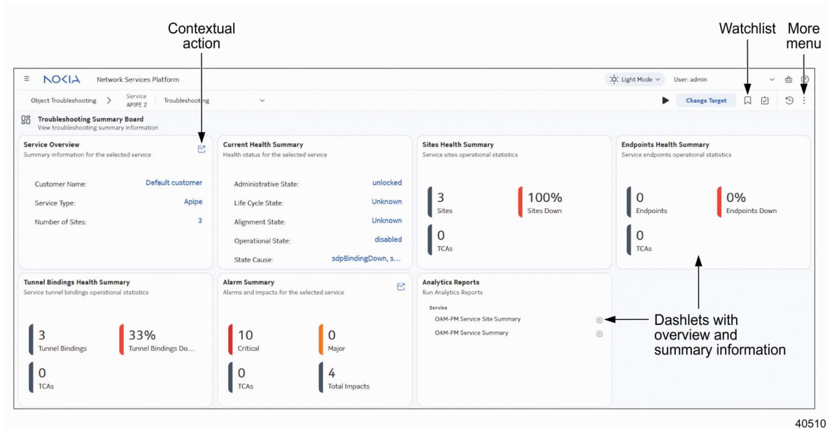
Figure 2-5 Dashboard overview
