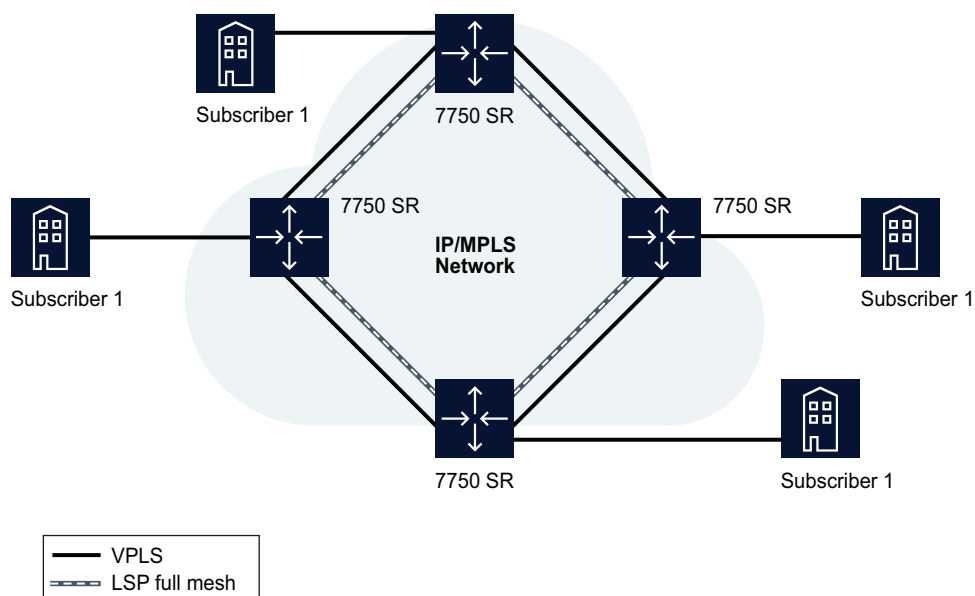
Figure 70-2 Distributed VPLS
