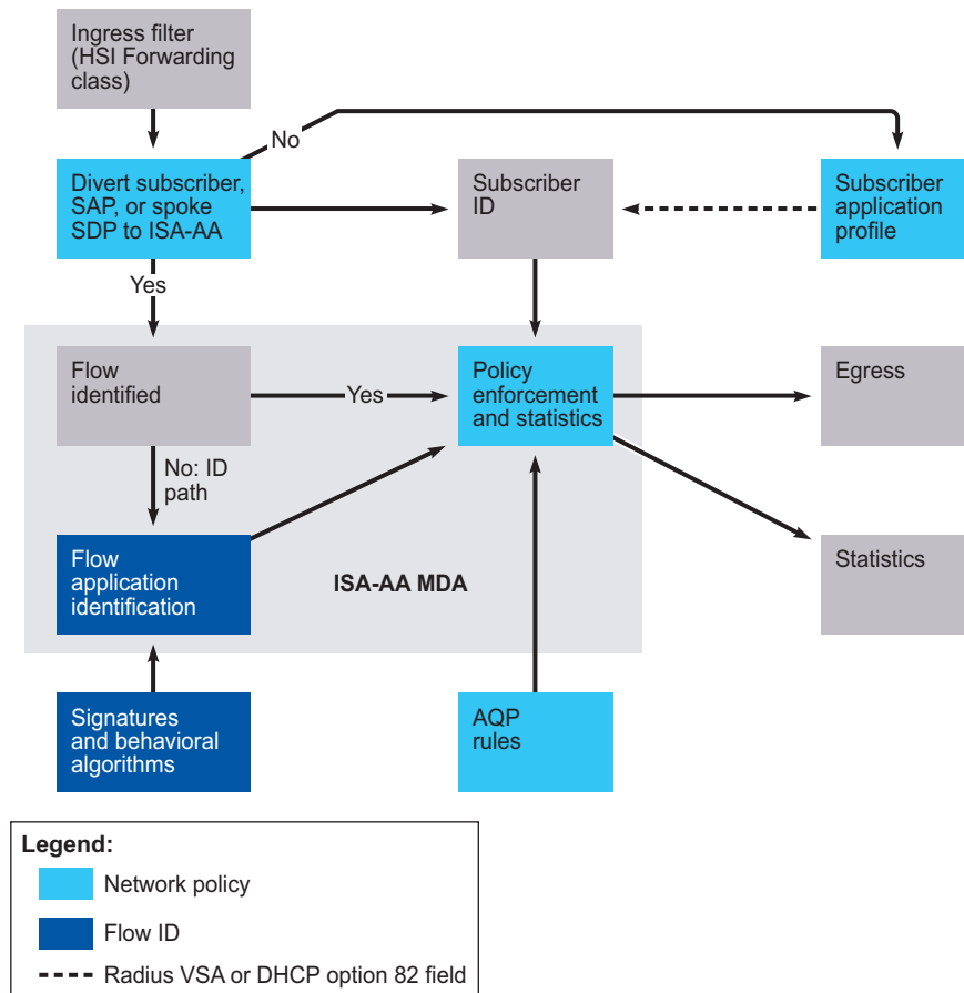
Figure 87-1 AA components
