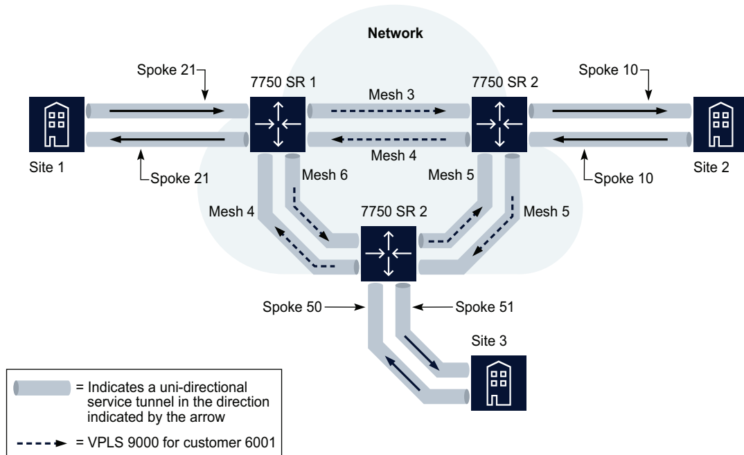
Figure 77-1 HVPLS configuration
