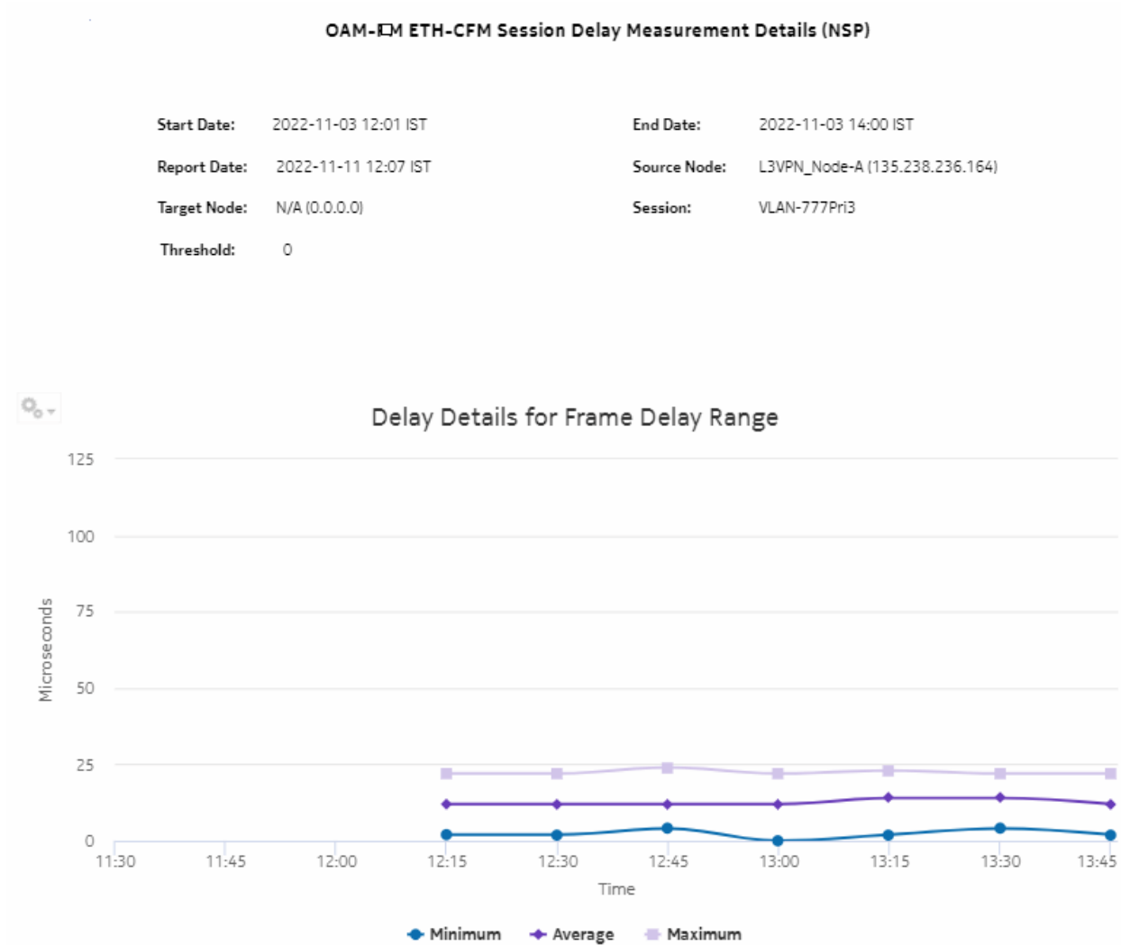
Figure 18-9 OAM-PM ETH-CFM Session Delay Measurement Details (NSP) – Delay Details for Frame Delay Range
