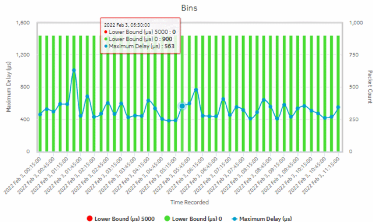
Figure 18-4 OAM-PM Bins and Delay (NSP) report – NFM-P NE CFM DMM session bins and delay
