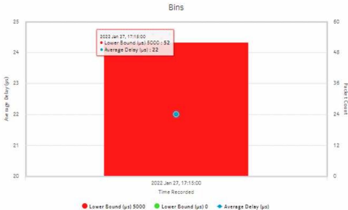
Figure 18-6 OAM-PM Bins and Delay (NSP) report – MDM NE CFM DMM light session bins and delay
