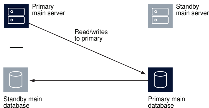
Figure 16-10 Server and database roles after database reinstantiation
