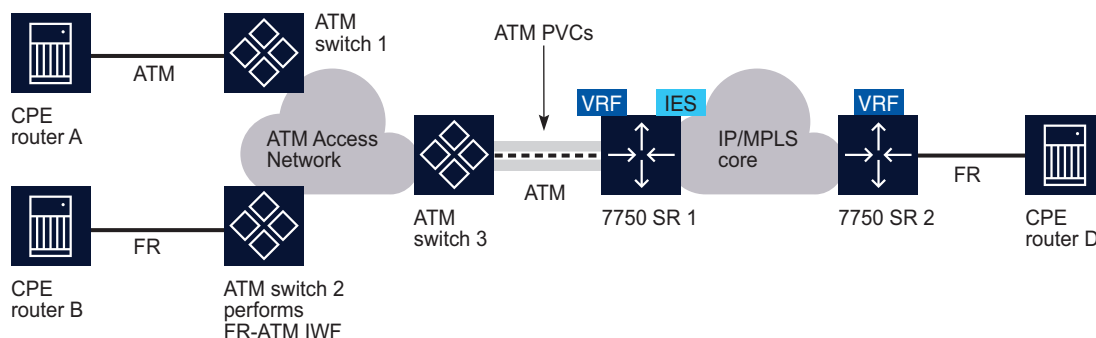
Figure 79-2 ATM SAP network connection to a VPRN
