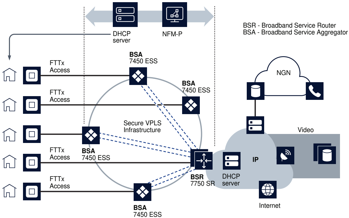
Figure 70-13 TPSDA components
