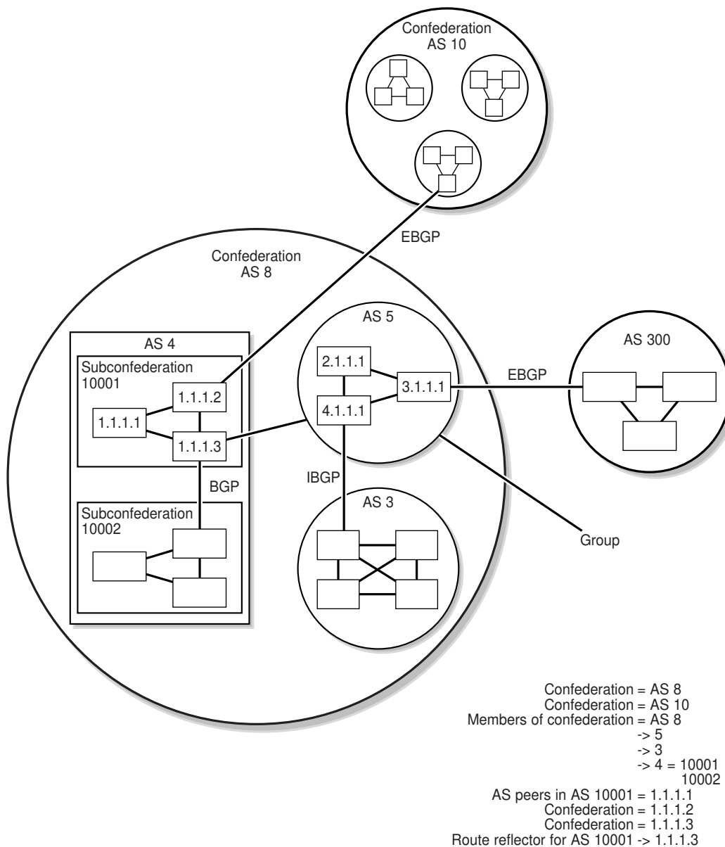
Figure 28-1 BGP example
