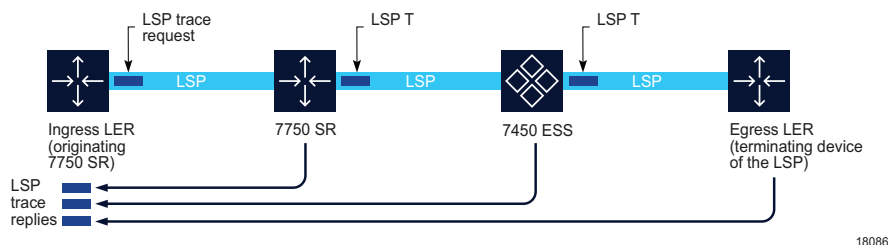
Figure 90-6 LSP Trace diagnostic test
