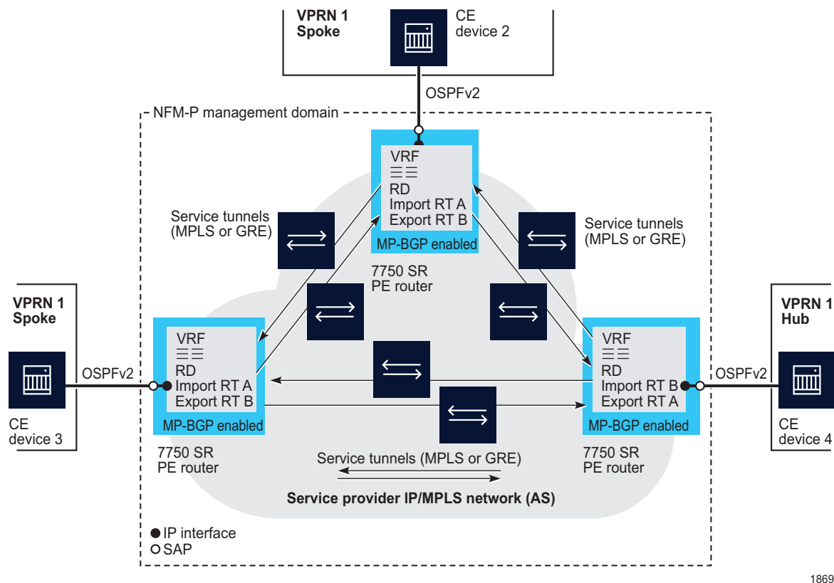
Figure 79-5 Sample hub-and-spoke VPRN Configuration
