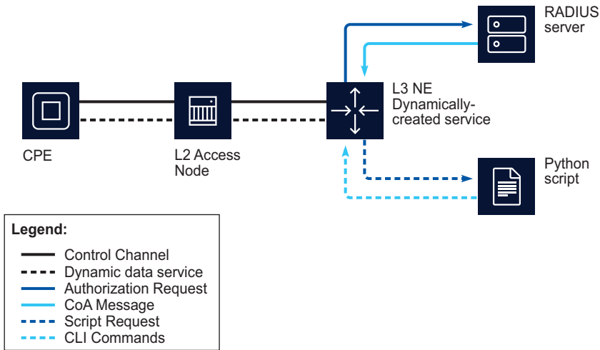
Figure 86-1 Basic dynamic service
