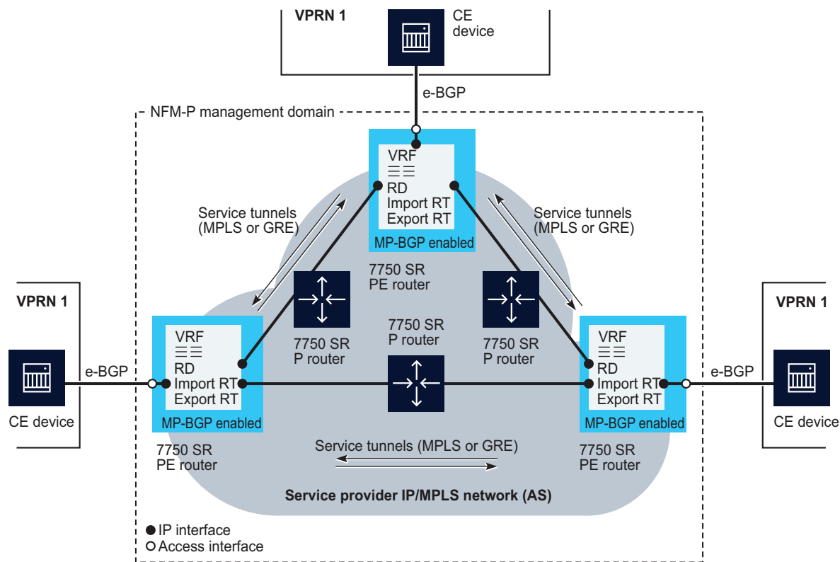
Figure 79-4 Sample VPRN Configuration
