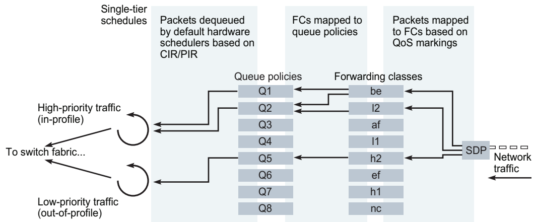
Figure 70-10 Network and network queue policy elements on ingress
