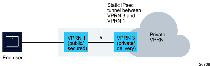
Figure 34-1 Static IPsec tunnel
