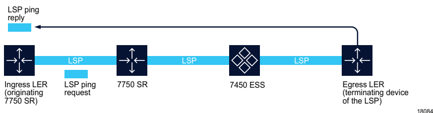
Figure 90-5 LSP ping OAM diagnostic test
