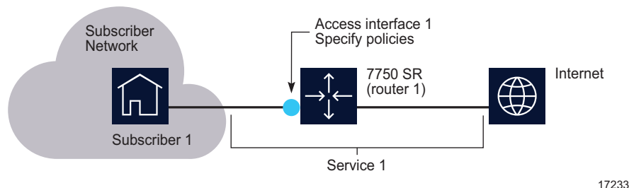
Figure 78-3 Sample IES configuration
