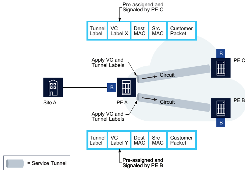
Figure 77-14 Packet forwarding from PE A across the core IP/MPLS network
