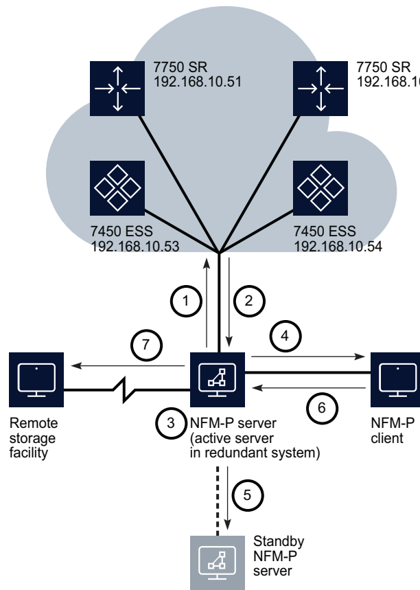
Figure 23-1 NFM-P backup process
