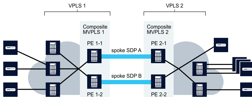
Figure 77-2 Composite MVPLS
