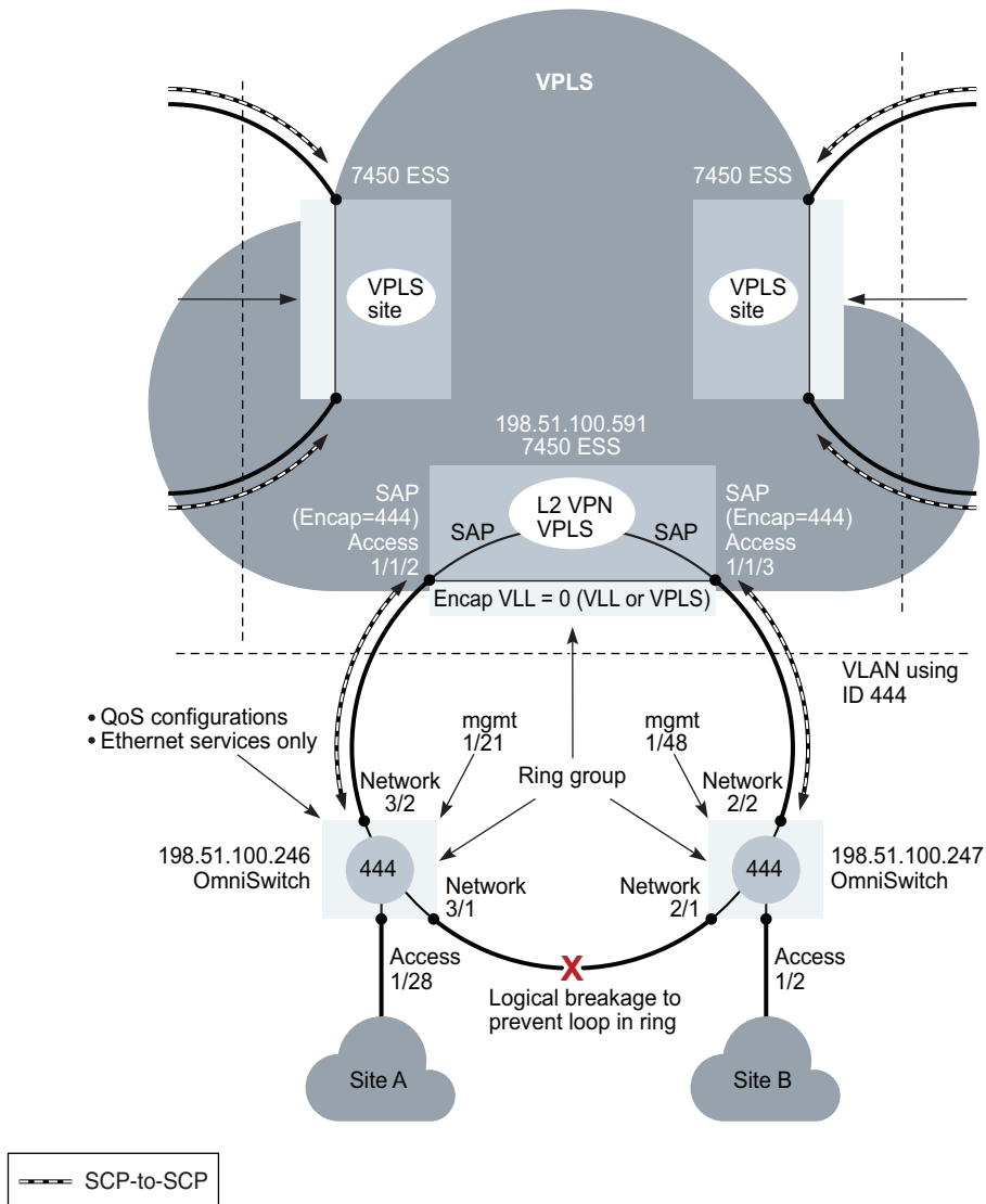
Figure 75-4 Sample interconnection VLAN
