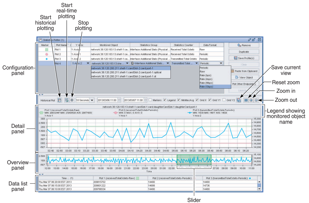
Figure 9-1 NFM-P Statistics Plotter
