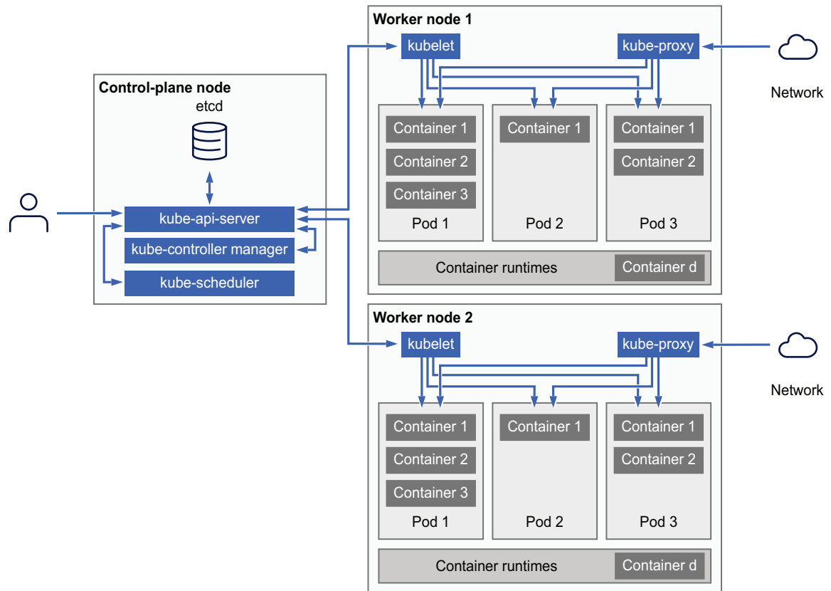
Figure 5-2 Kubernetes cluster
