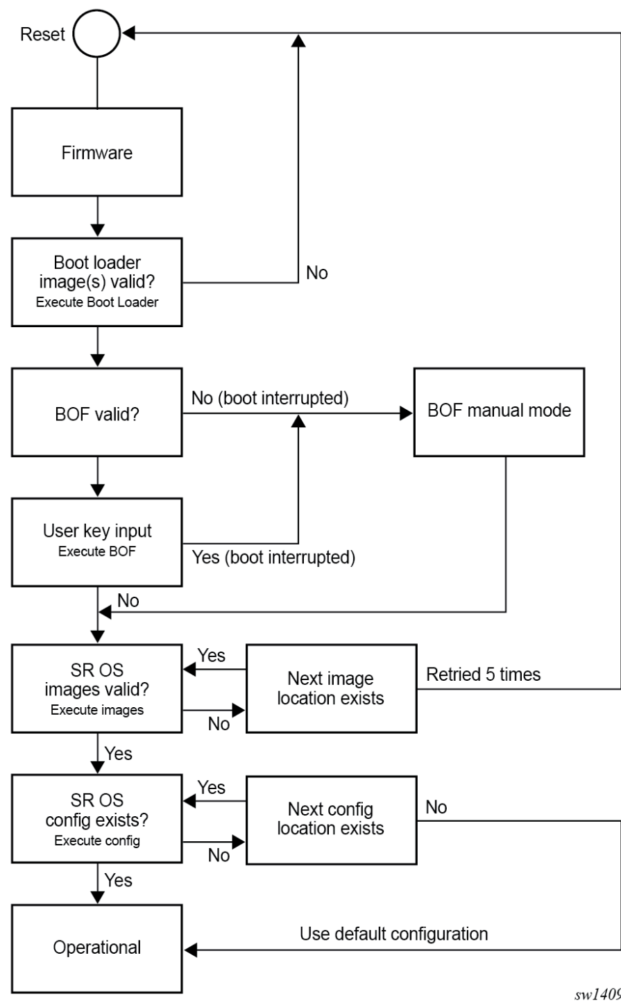
Figure 1: Boot process
