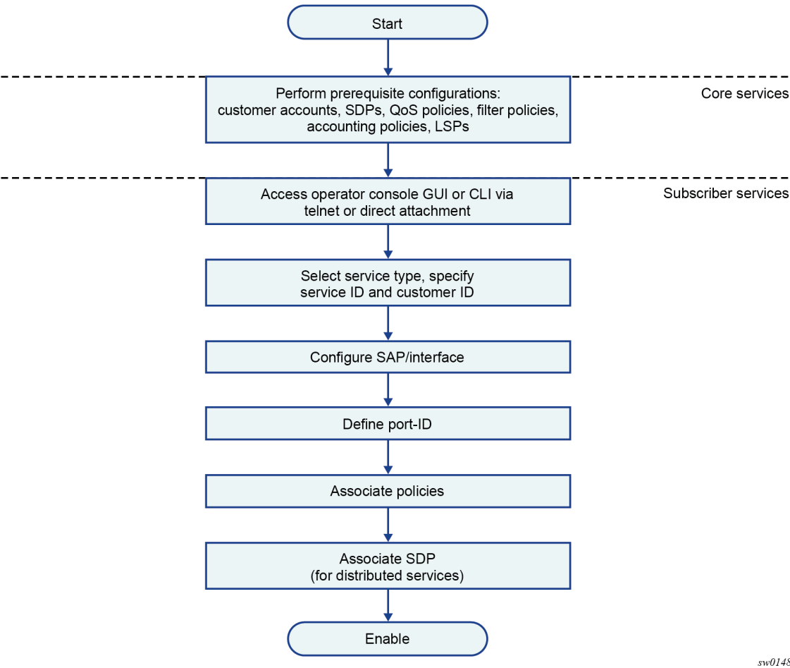
Figure 29: Service creation and implementation flow
