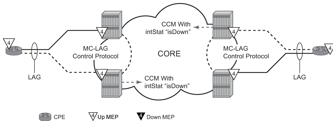
Figure 33: Independent processing up MEP example
