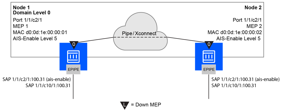
Figure 31: Port-Based MEP example
