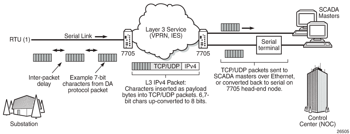
Figure 26: TCP/UDP packet transport over IP/MPLS
