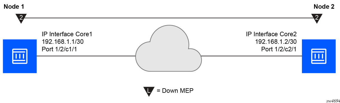
Figure 32: Router MEP example
