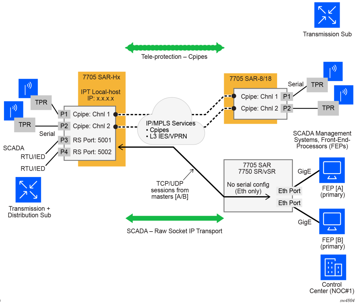
Figure 28: Raw socket and Cpipe support on the 7705 SAR Gen
