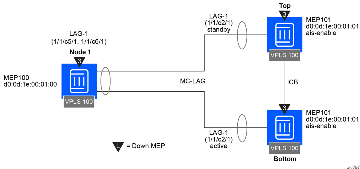
Figure 35: ETH-CFM and MC-LAG example
