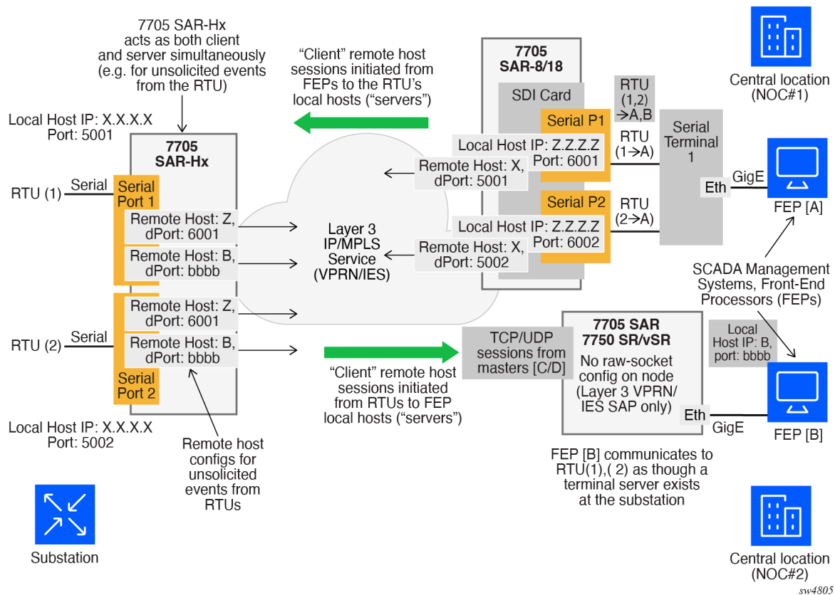
Figure 25: IP transport service
