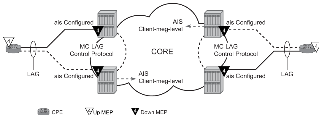
Figure 34: Independent processing down MEP example
