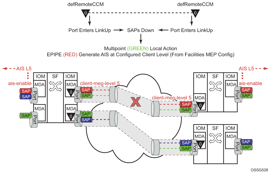
Figure 30: Fault handling non-member port
