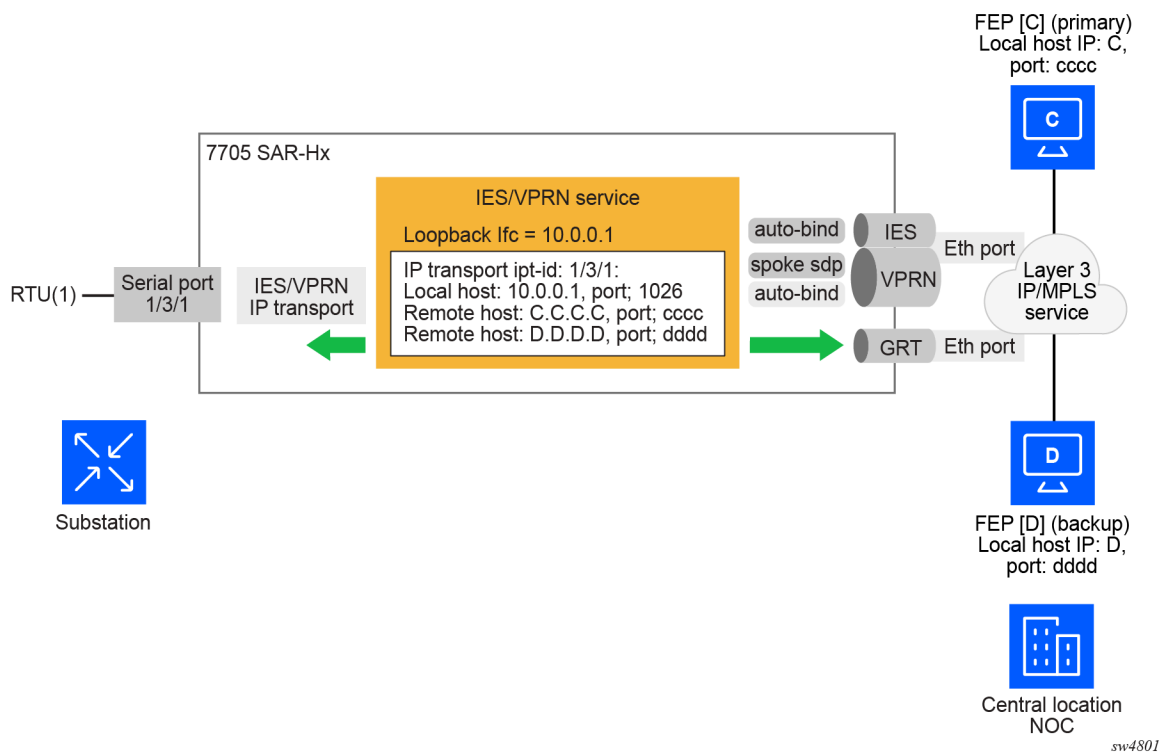
Figure 27: IES/VPNR IP transport service
