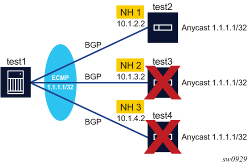
Figure 22: Sticky ECMP flow distribution as next hops are removed (part 3)
