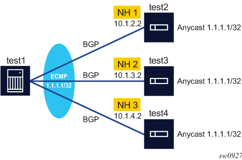
Figure 21: Sticky ECMP flow distribution as next hops are removed (part 2)
