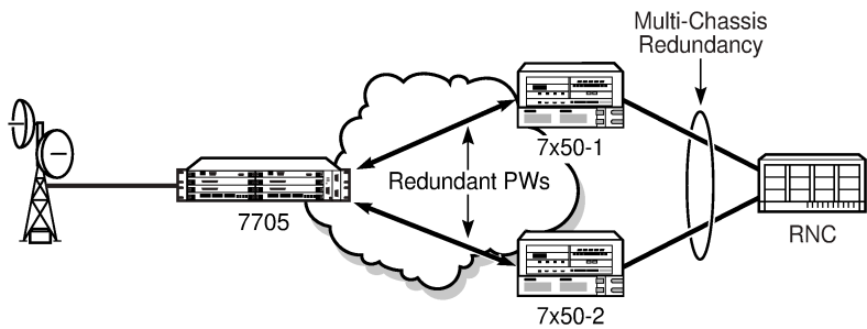
Figure 17: Pseudowire redundancy
