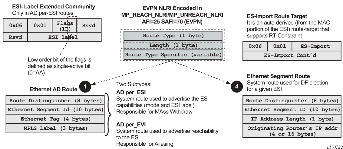
Figure 89: EVPN routes type 1 and 4
