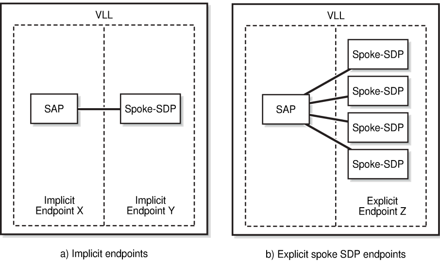
Figure 18: Implicit and explicit endpoint objects
