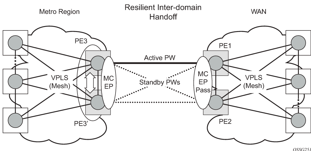
Figure 40: MC-EP in passive mode
