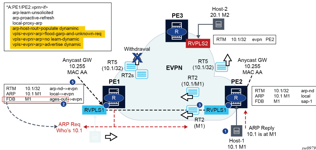
Figure 122: Host mobility within the same R-VPLS – silent host
