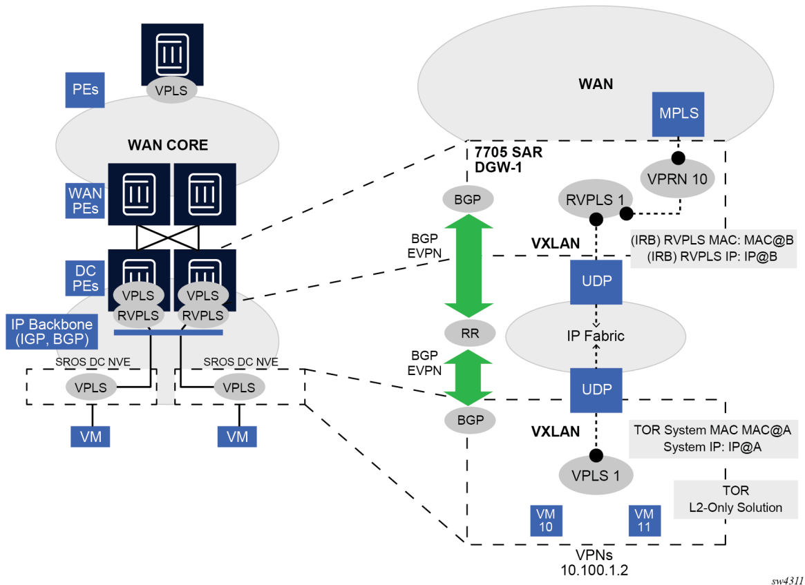
Figure 71: Gateway IRB on the DC PE for an L2 EVPN/VXLAN DC
