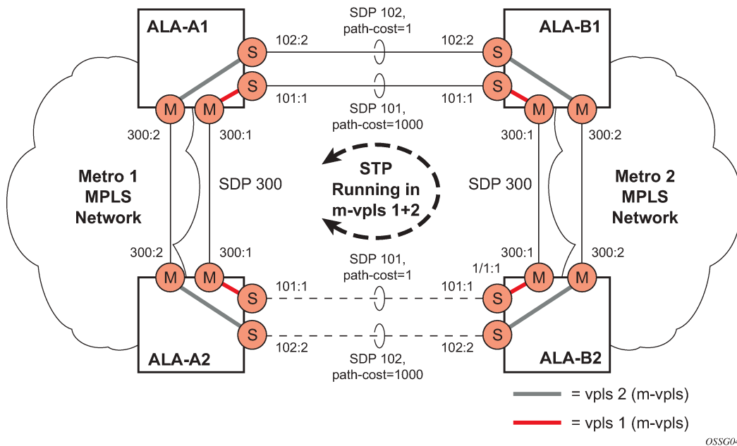
Figure 62: Example configuration for load balancing across two protected VPLS spoke-SDPs
