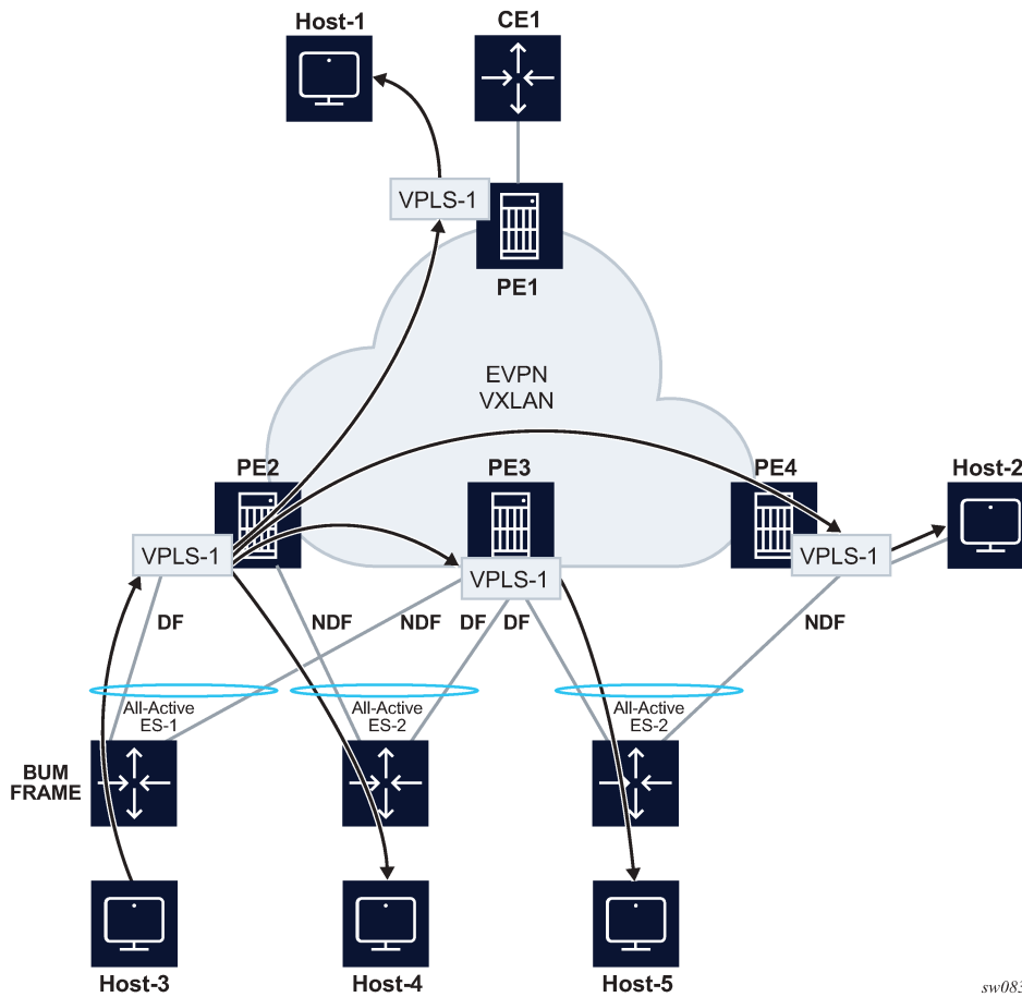
Figure 85: EVPN-VXLAN multihoming with local bias
