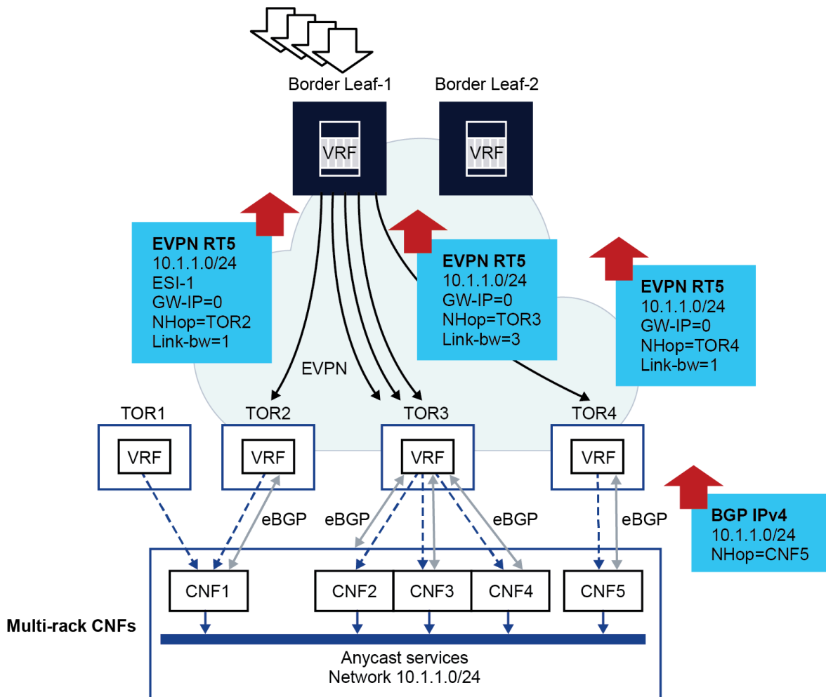
Figure 138: Weighted ECMP for IP Prefix routes use case
