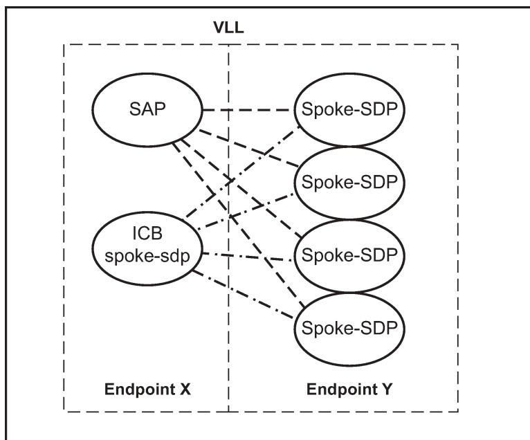
Figure 7: Redundant VLL endpoint objects
