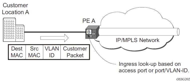
Figure 28: Access port ingress packet format and lookup
