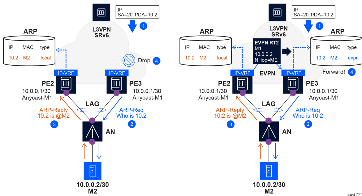
Figure 141: Comparing network behavior with EVPN ARP-ND synchronization on Layer 3 interfaces disabled or enabled
