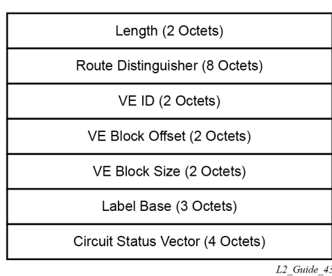
Figure 13: BGP VPWS NLRI
