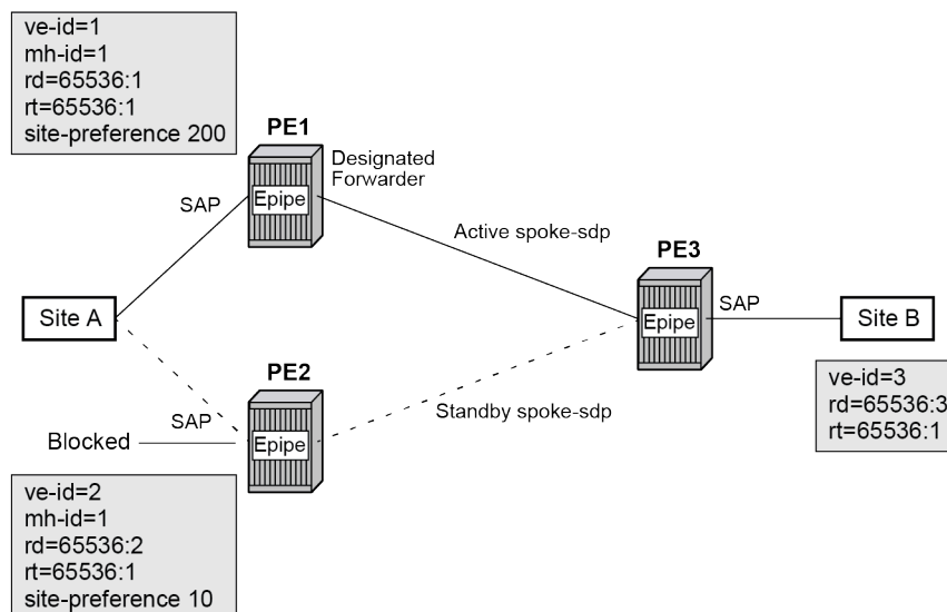
Figure 10: Dual-homed BGP VPWS with active/standby pseudowires
