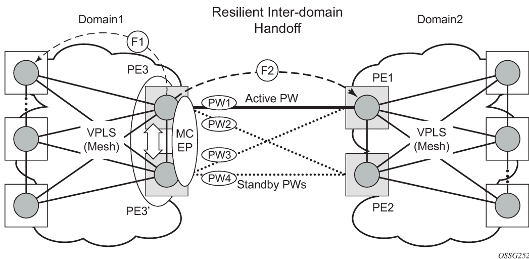
Figure 41: MAC flush in the MC-EP solution
