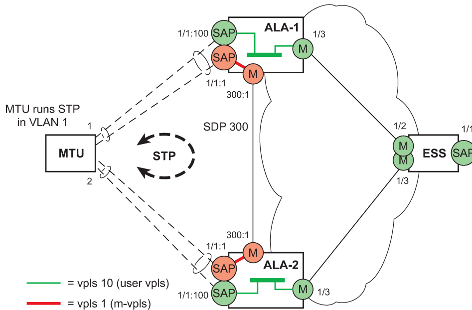
Figure 60: Example configuration for protected VPLS SAP
