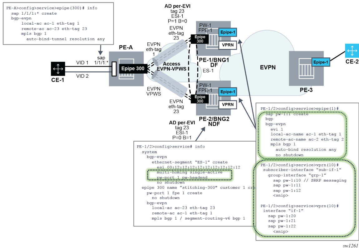
Figure 128: ES FPE-based pw-port headend
