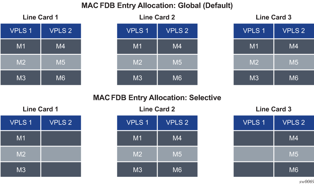
Figure 33: MAC FDB entry allocation: global versus selective
