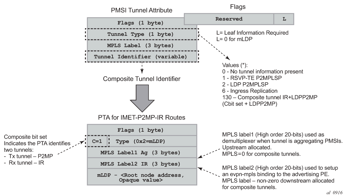
Figure 88: Composite p2mp mLDP and IR tunnels—PTA
