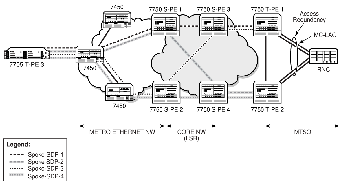
Figure 19: Pseudowire redundancy with four spoke SDPs
