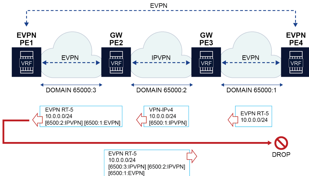
Figure 132: D-PATH attribute example
