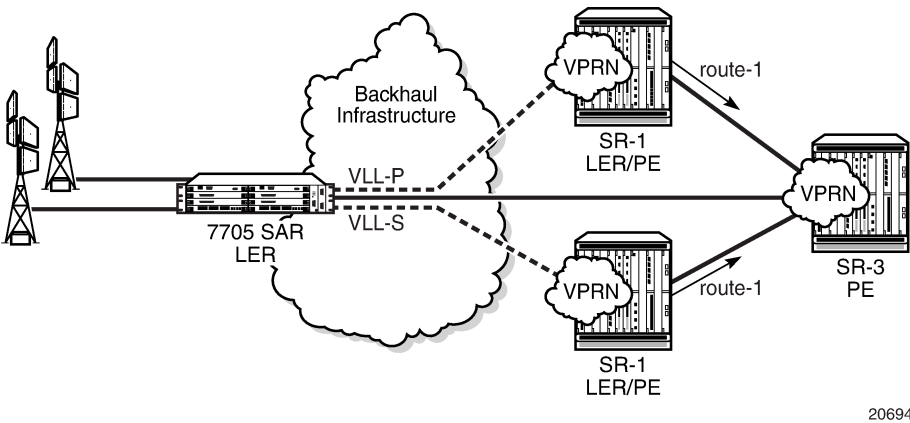
Figure 20: Active/standby mode for redundant pseudowires
