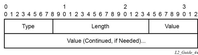
Figure 15: Circuit status vector TLV type
