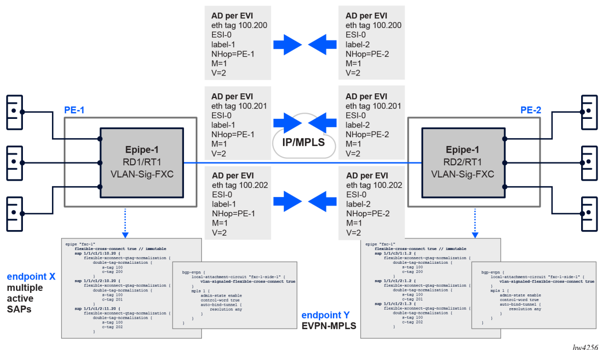
Figure 97: VLAN-aware bundle or VLAN-signaled FXC mode
