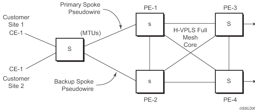
Figure 42: Dual-homed MTUs in two-tier hierarchy H-VPLS
