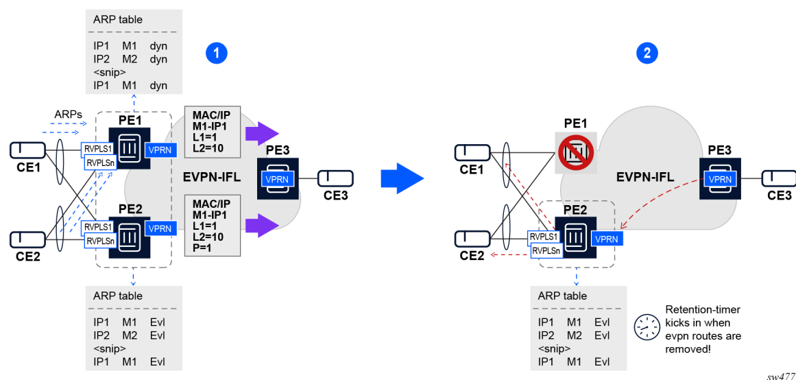
Figure 140: Comparing two states in the same multihoming network with EVPN local ES configured
