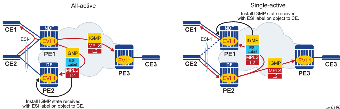
Figure 99: Data-driven IGMP snooping synchronization with EVPN multihoming
