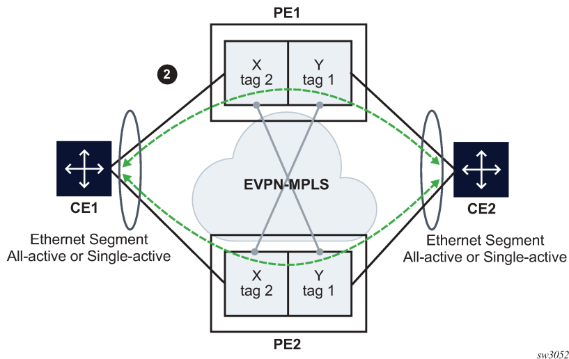
Figure 94: EVPN-VPWS endpoints example 2
