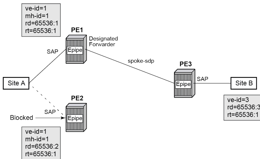
Figure 9: Dual-homed BGP VPWS with single pseudowire
