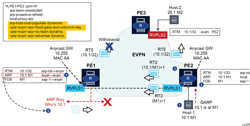
Figure 120: Host mobility within the same R-VPLS – move with GARP
