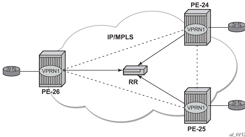
Figure 68: BGP VPLS example
