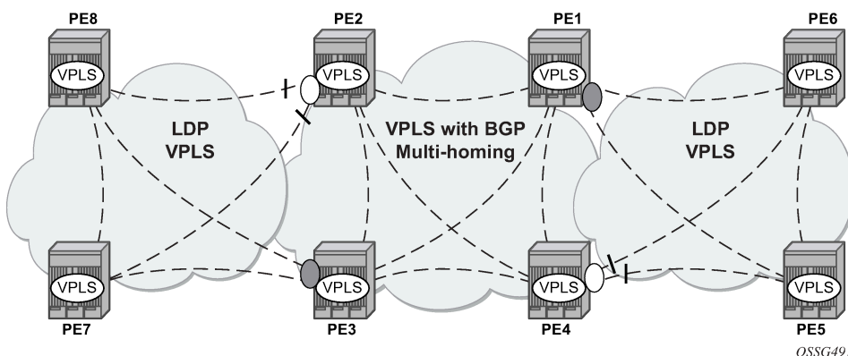
Figure 54: BGP MH used in an HVPLS topology
