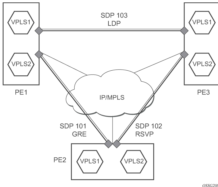
Figure 16: SDP statistics for VPLS and VLL services
