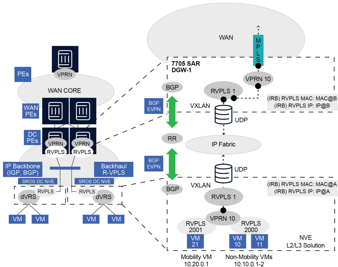
Figure 72: Gateway IRB on the DC PE for an L3 EVPN/VXLAN DC
