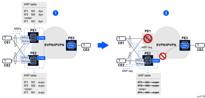
Figure 139: Comparing two states in the same multihoming network
