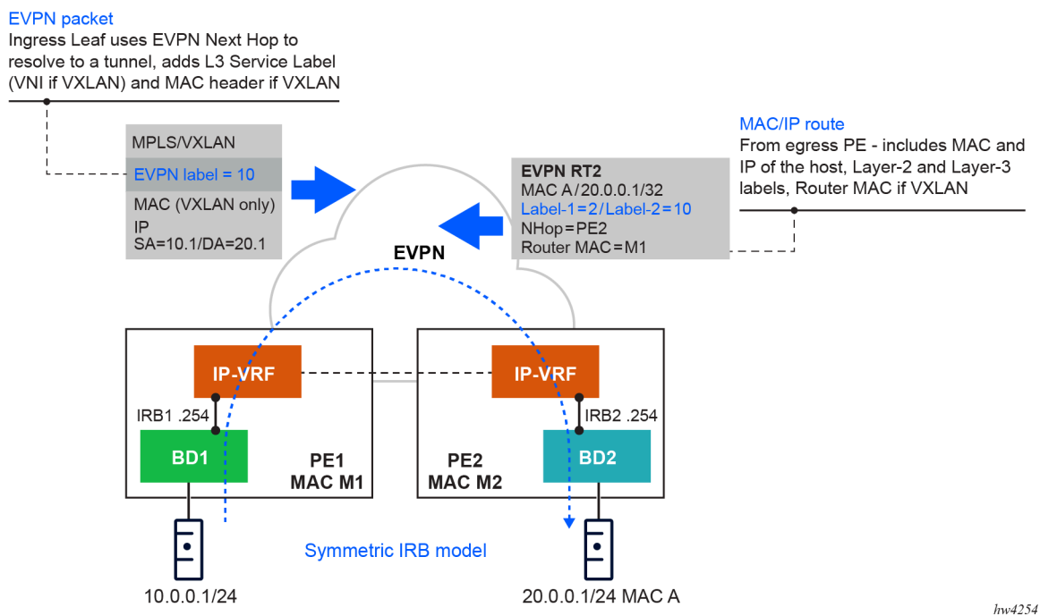
Figure 117: Symmetric IRB model
