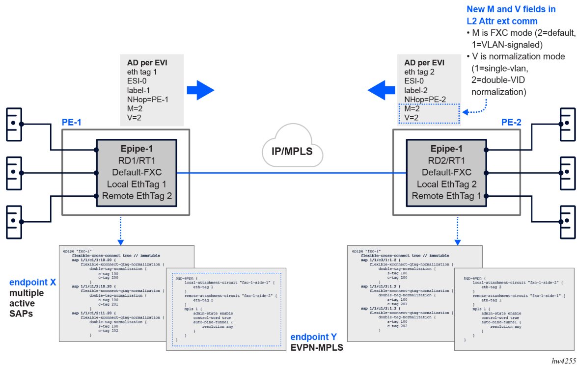
Figure 96: Default FXC mode
