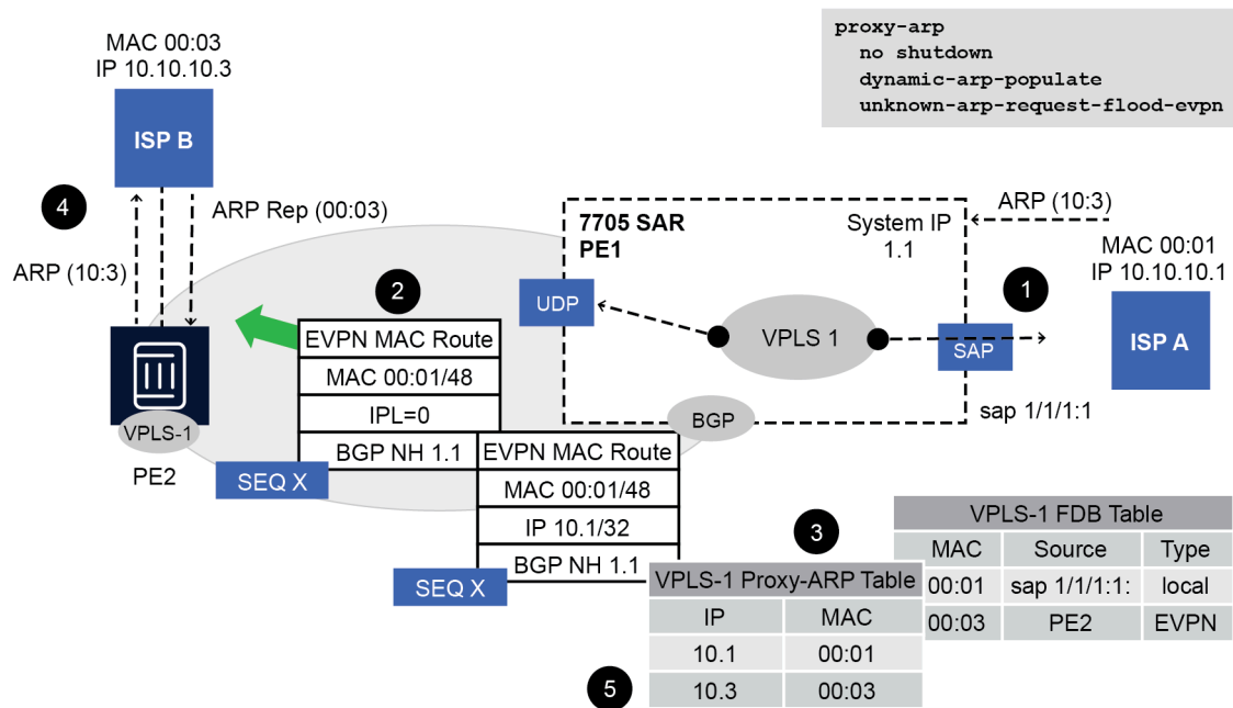
Figure 103: Proxy-ARP example usage in an EVPN network
