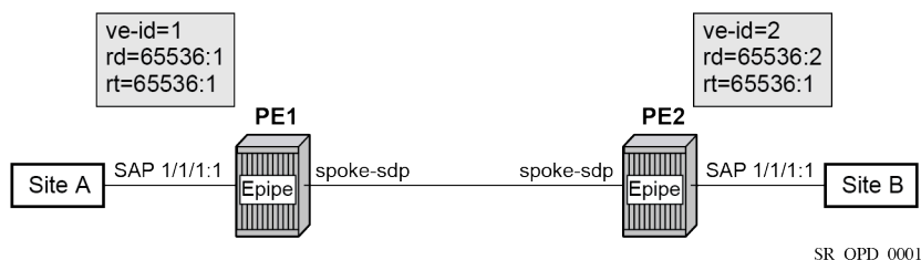
Figure 8: Single-homed BGP-VPWS example
