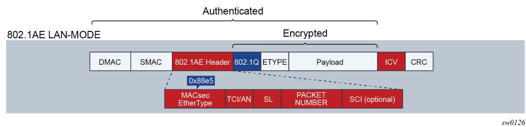
Figure 4: 802.1 AE LAN-MODE
