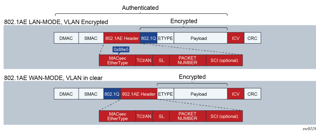
Figure 6: 802.1 AE LAN and WAN modes and VLAN encrypted and cleartext
