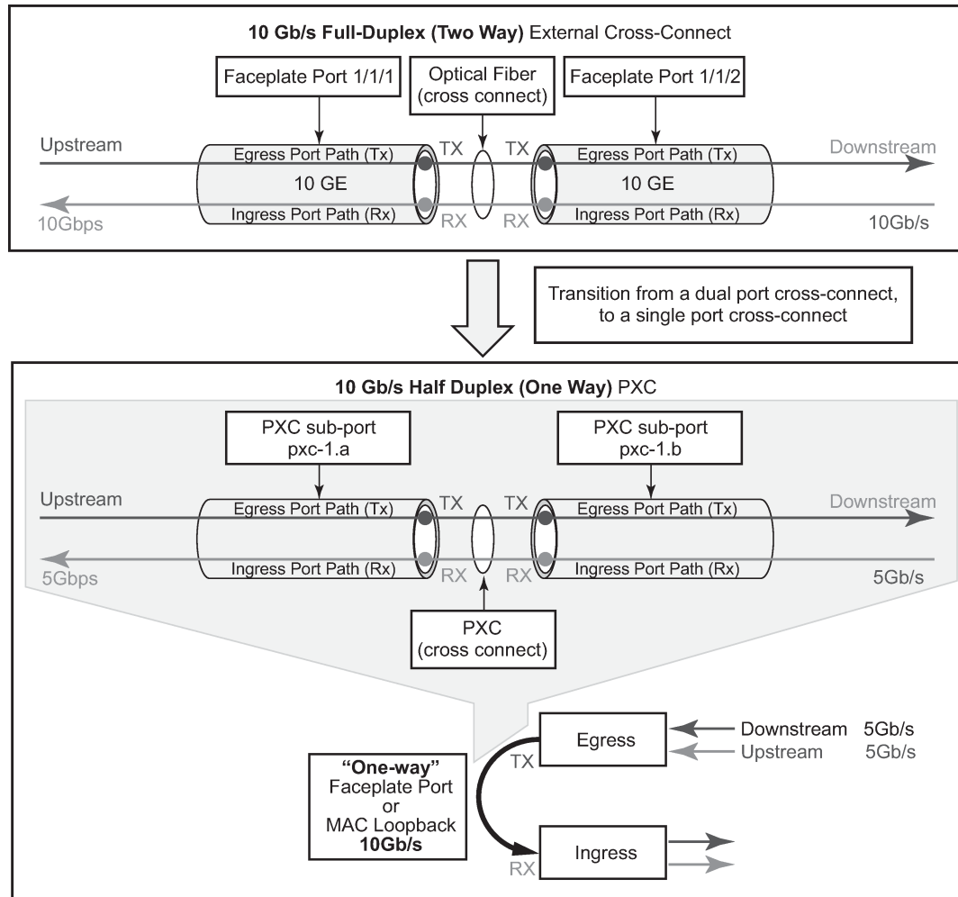
Figure 17: Two cross-connected external ports versus a single cross-connect
