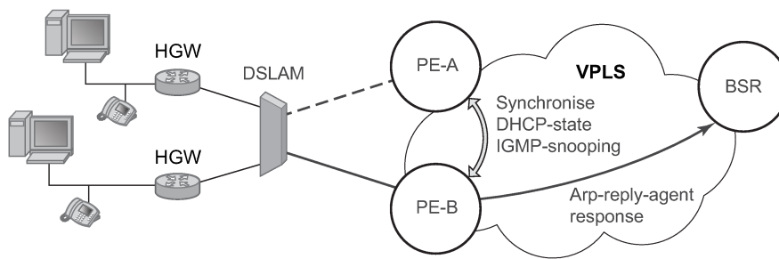
Figure 31: DSLAM dual-homing using MC-LAG
