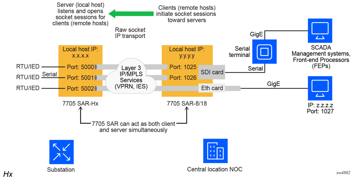
Figure 32: Serial transport over raw socket application on the 7705 SAR-
