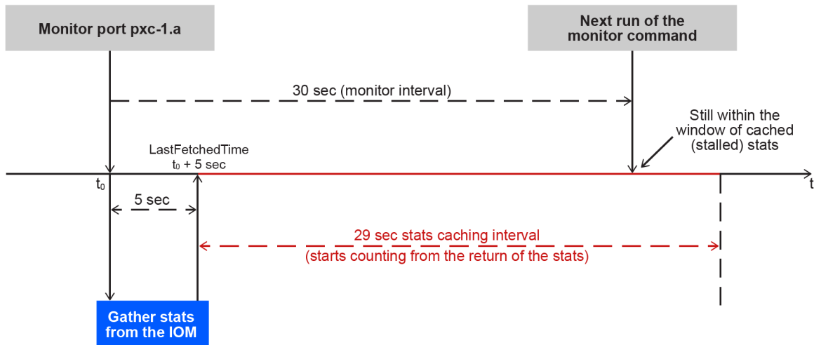
Figure 20: Monitor port interval issue
