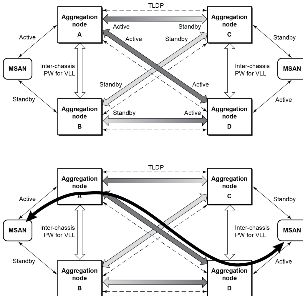
Figure 30: Point-to-Point (P2P) redundant connection through a Layer 2 VPN network
