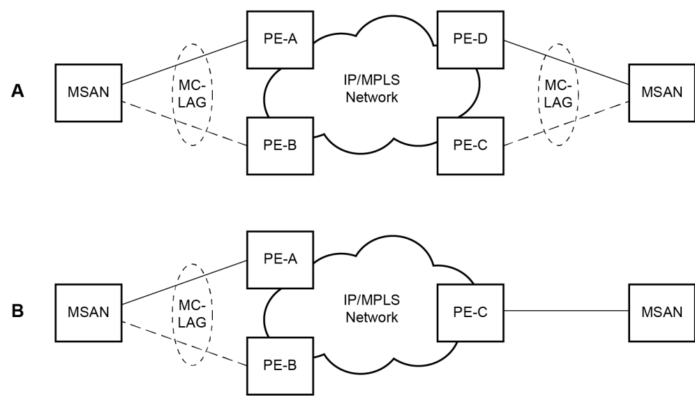
Figure 28: MC-LAG Layer 2 dual-homing to remote PE pairs
