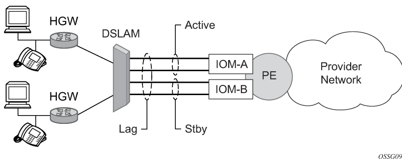
Figure 26: LAG on access failure switchover
