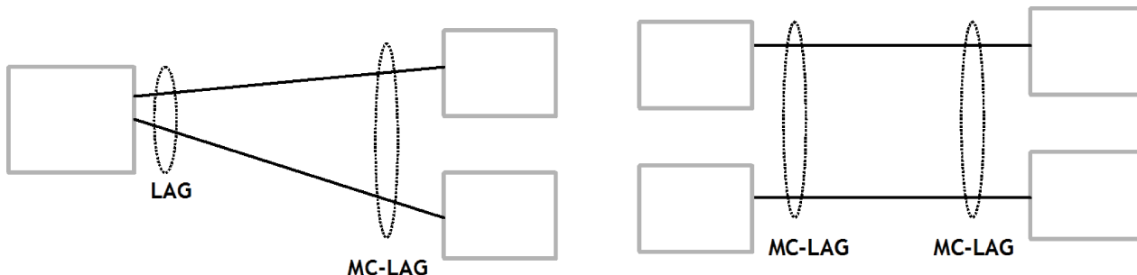
Figure 24: Active/standby LAG operation deployment examples
