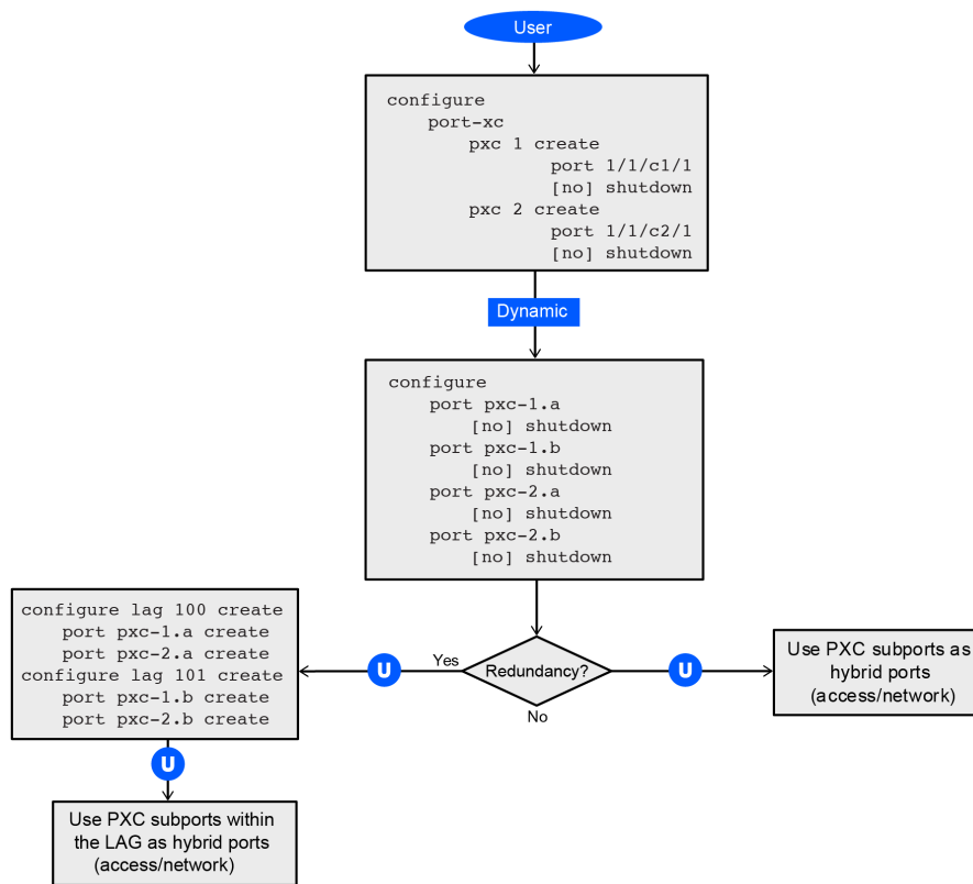
Figure 23: Classic CLI flow
