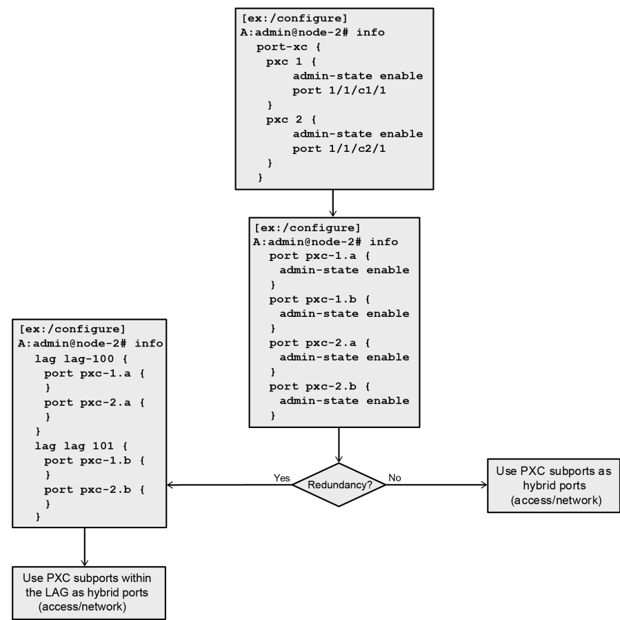
Figure 22: MD-CLI flow
