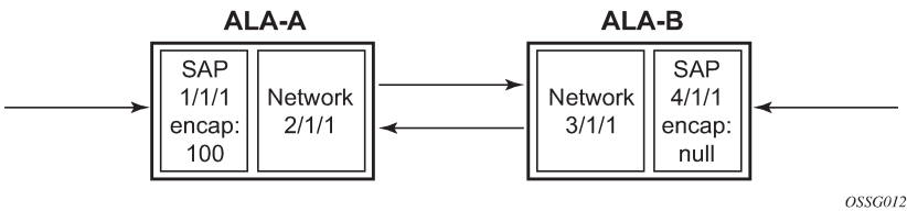
Figure 34: MTU configuration example
