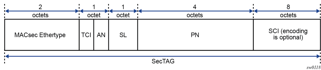
Figure 5: SecTAG format
