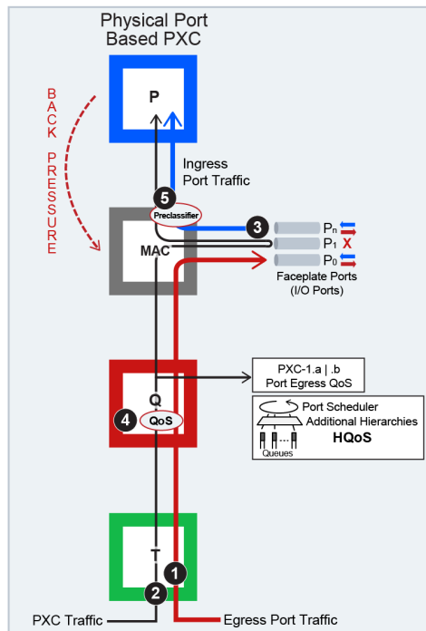
Figure 18: Interaction between PXC and non-PXC traffic
