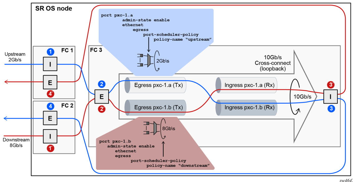
Figure 19: Bandwidth management on PXC sub-ports
