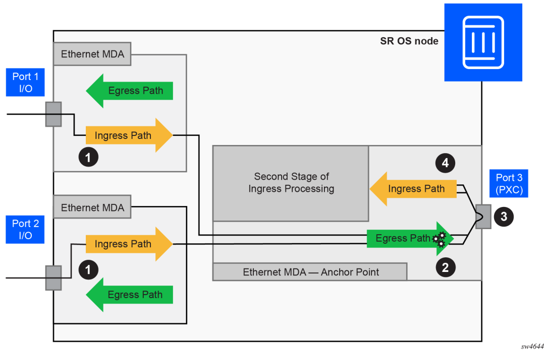
Figure 15: Traffic preprocessing using PXC
