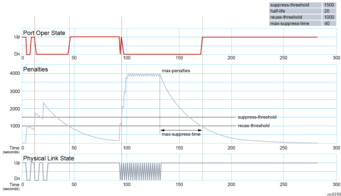
Figure 14: EPD example
