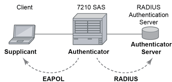
Figure 1: 802.1x architecture
