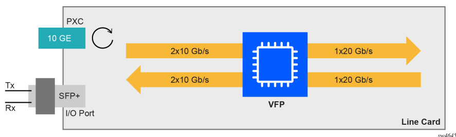
Figure 16: Port-based PXC
