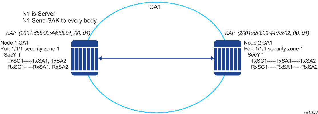
Figure 12: Switch-point to switch-point topology
