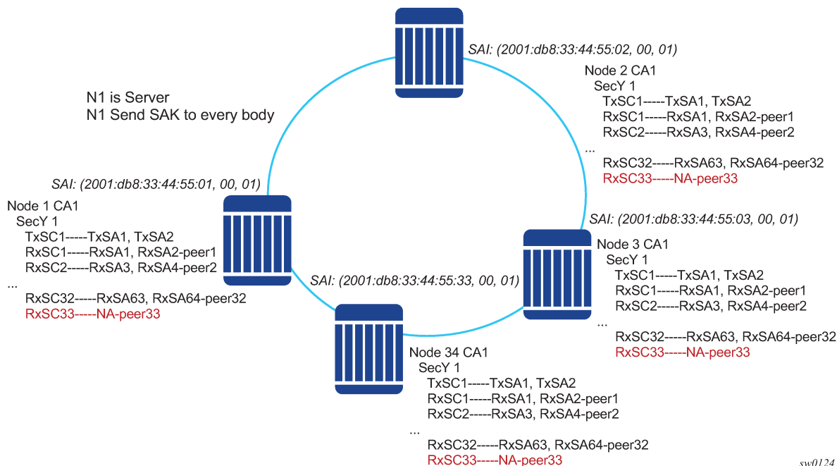
Figure 13: Switch-multipoint to switch-multipoint topology
