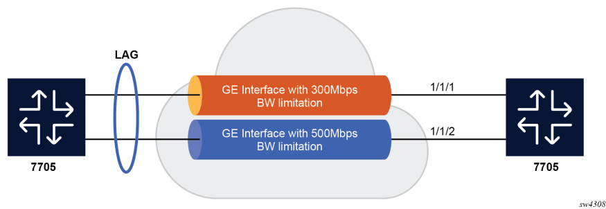
Figure 27: Same-speed LAG with ports of different hash weight
