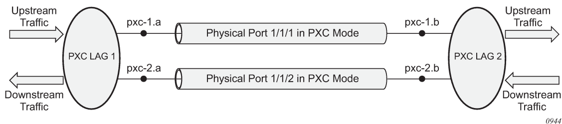
Figure 21: Logical concept of a LAG on PXC ports
