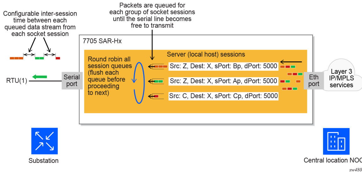
Figure 33: Raw socket packet processing
