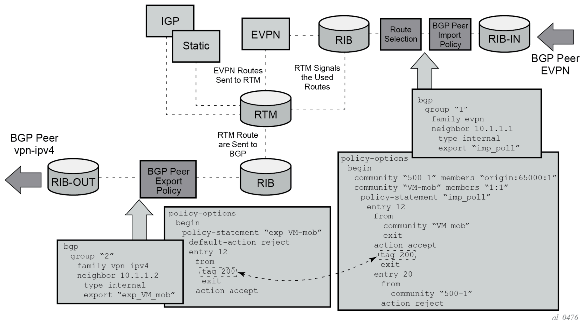
Figure 138: EVPN import and I-VPN export BGP workflow
