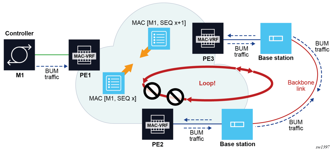
Figure 106: EVPN non-intrusive loop detection mechanism
