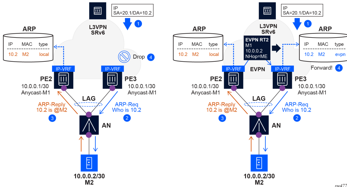
Figure 143: Comparing network behavior with EVPN ARP-ND synchronization on Layer 3 interfaces disabled or enabled
