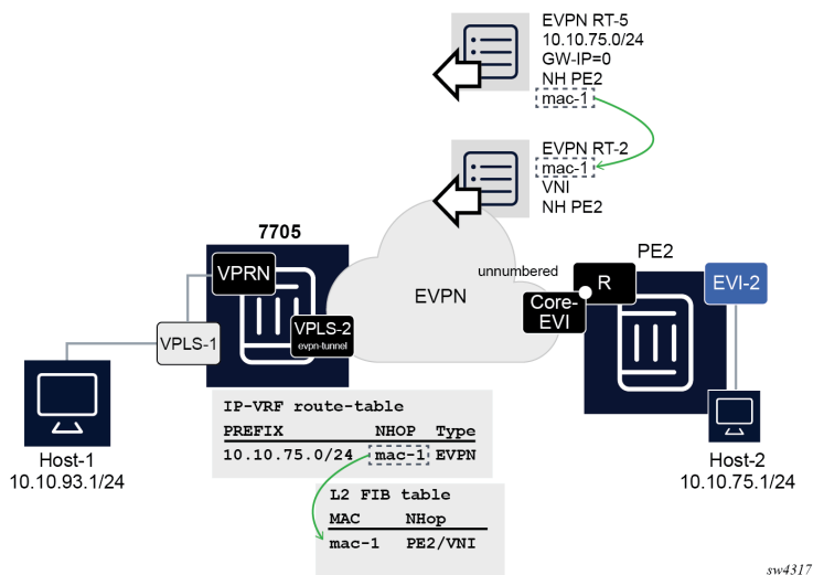
Figure 115: Interface-ful IP-VRF-to-IP-VRF with unnumbered SBD IRB model
