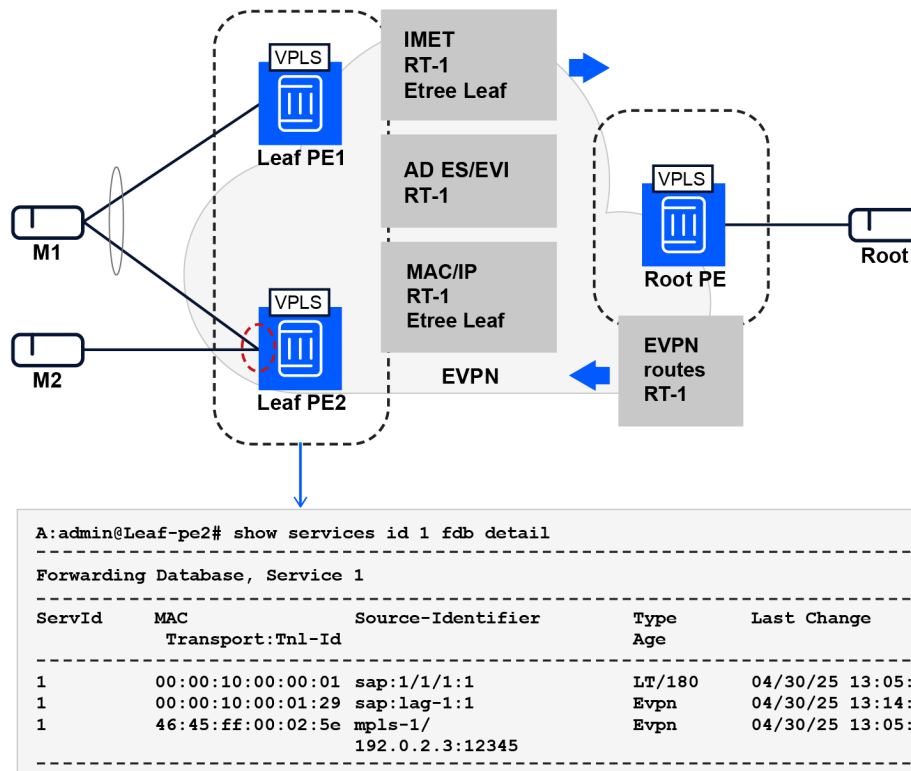
Figure 140: MAC installed with a destination on the local SAP
