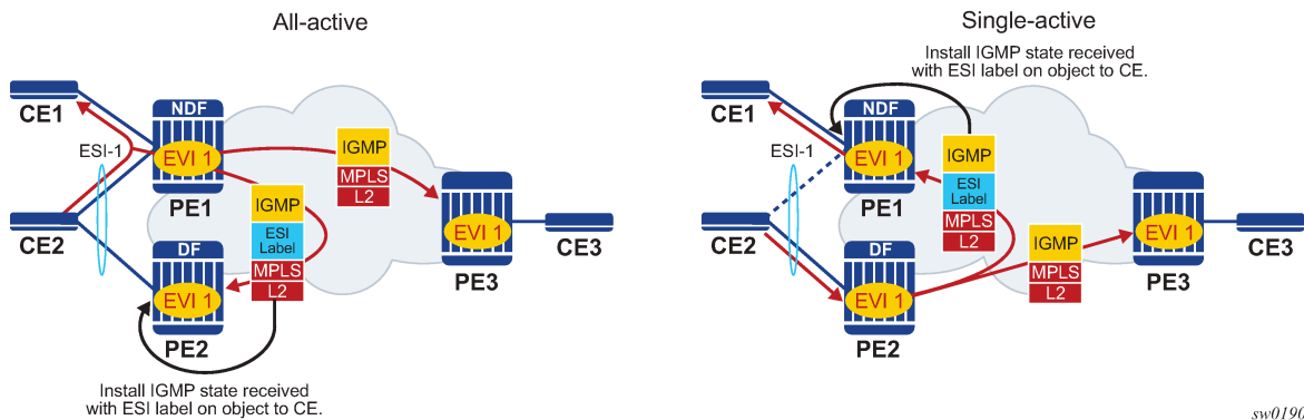
Figure 100: Data-driven IGMP snooping synchronization with EVPN multihoming
