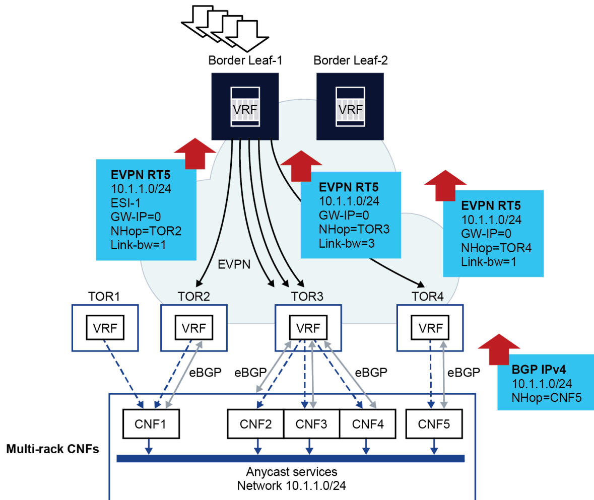
Figure 139: Weighted ECMP for IP Prefix routes use case
