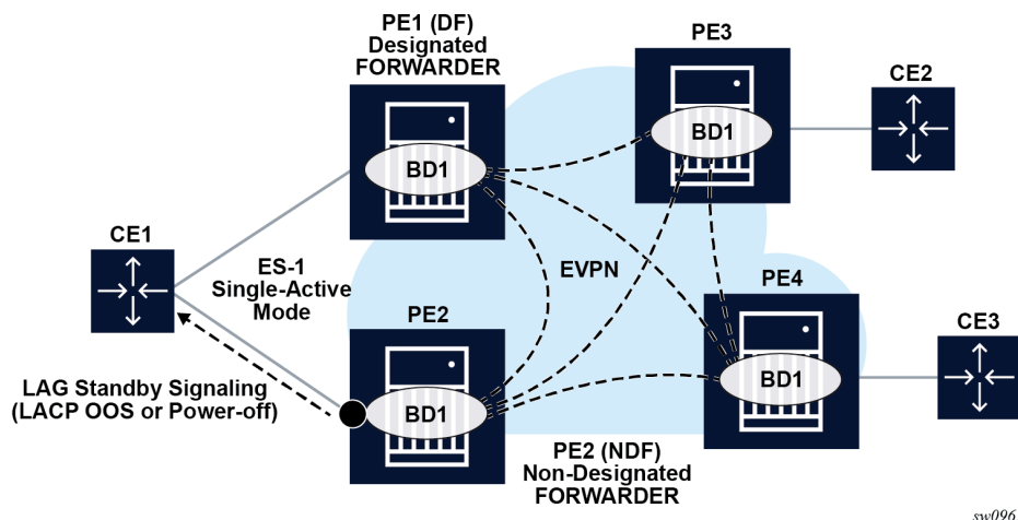
Figure 126: LACP standby signaling from the non-DF
