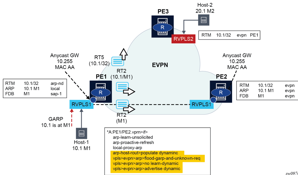
Figure 120: Host mobility within the same R-VPLS – initial phase
