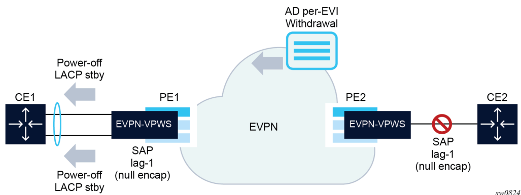
Figure 124: LLF for EVPN-VPWS
