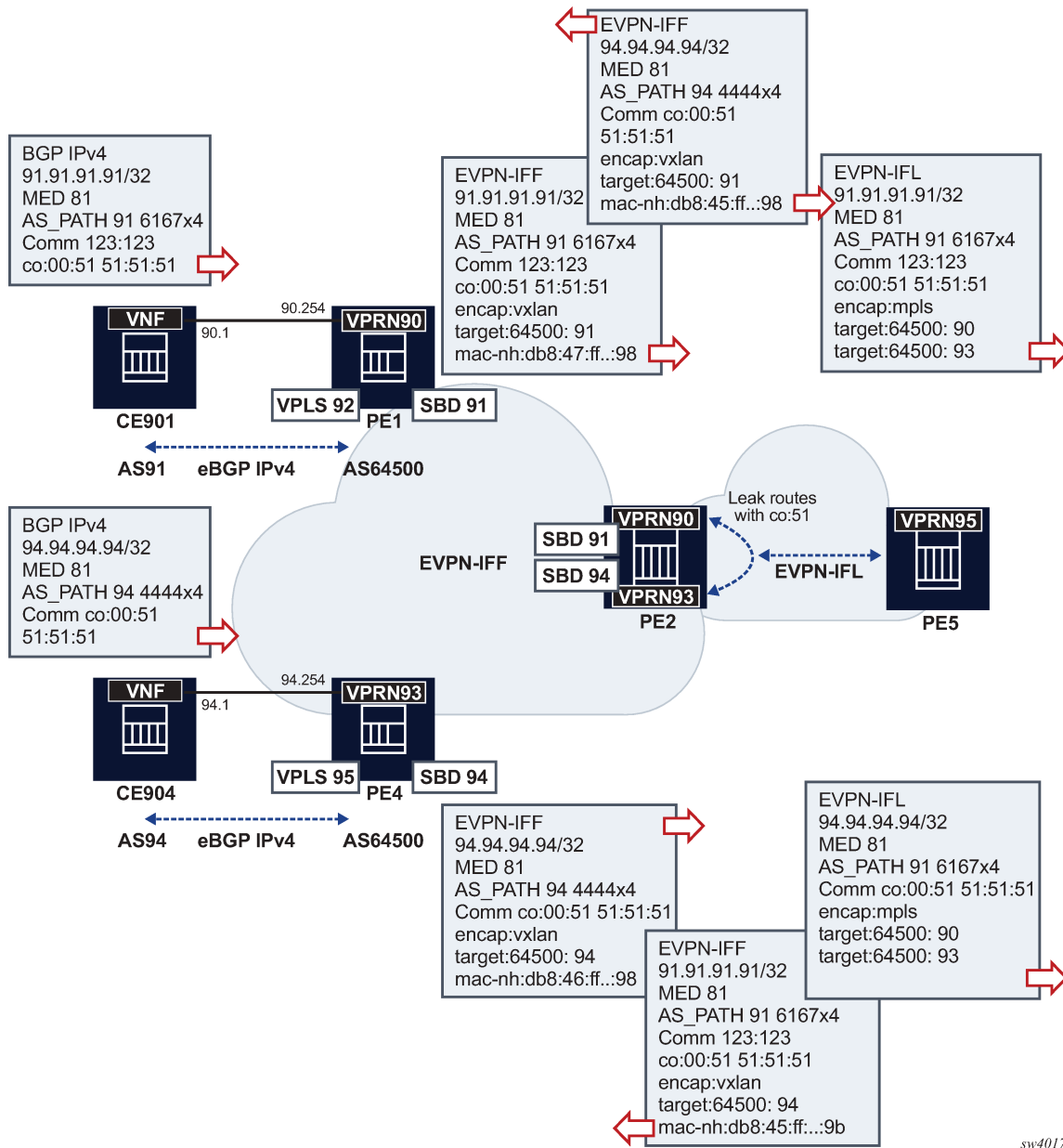
Figure 135: Propagation of BGP path attributes for EVPN-IFF
