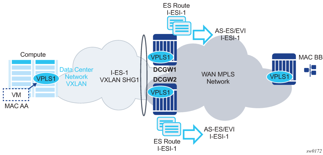
Figure 110: The Interconnect ES concept
