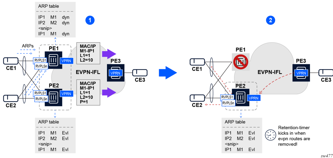
Figure 142: Comparing two states in the same multihoming network with EVPN local ES configured
