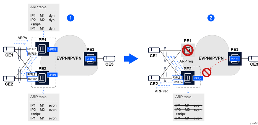
Figure 141: Comparing two states in the same multihoming network
