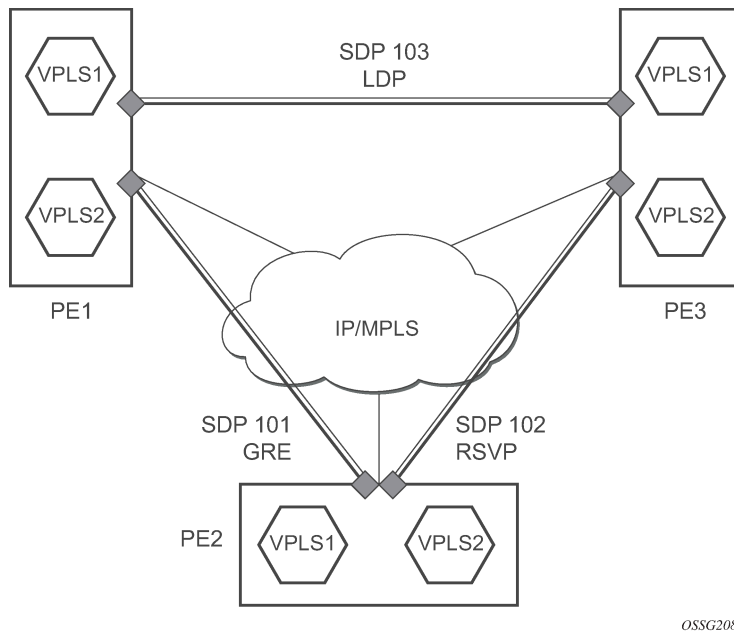
Figure 17: SDP statistics for VPLS and VLL services
