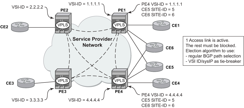
Figure 53: BGP multihoming for VPLS shows the VPLS using BGP multihoming for the case of multihomed CEs. Although the figure shows the case of a pseudowire infrastructure signaled with LDP for an LDP VPLS using BGP-AD for discovery, the procedures are identical for BGP VPLS or for a mix of BGP- and LDP-signaled pseudowires.
