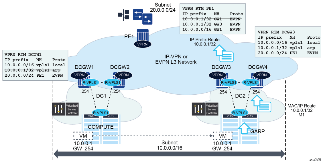
Figure 119: Extended Layer 2 data centers
