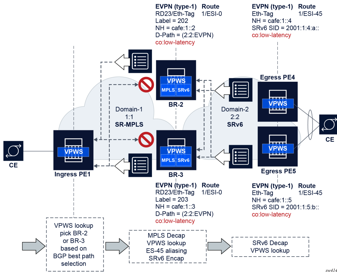
Figure 108: Multihomed anycast solution for Epipe services
