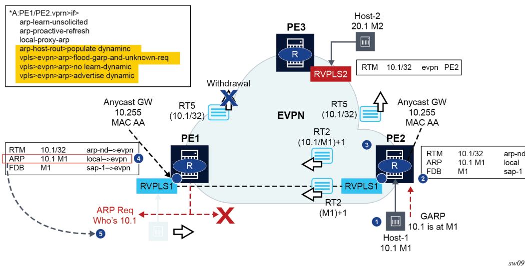
Figure 121: Host mobility within the same R-VPLS – move with GARP
