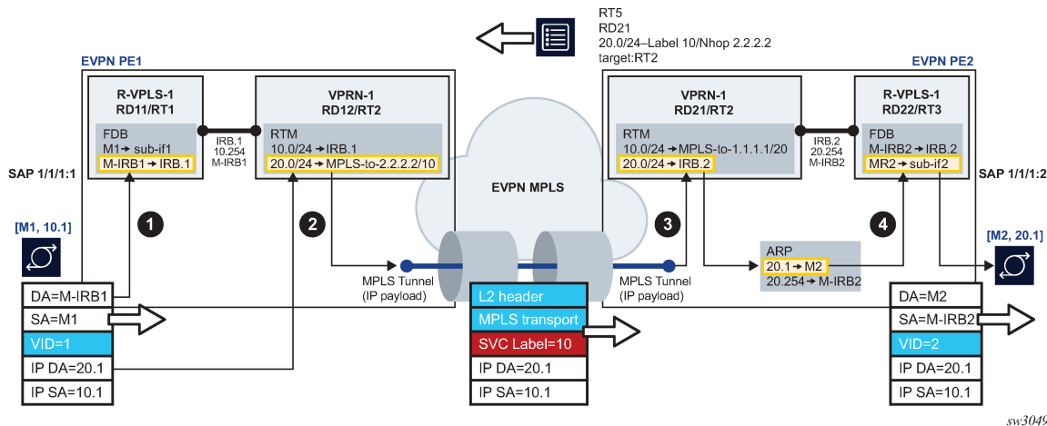
Figure 117: Interface-less IP-VRF-to-IP-VRF model for IP encapsulation in MPLS tunnels
