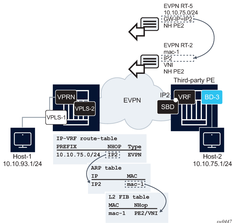
Figure 114: Interface-ful IP-VRF-to-IP-VRF with SBD IRB model
