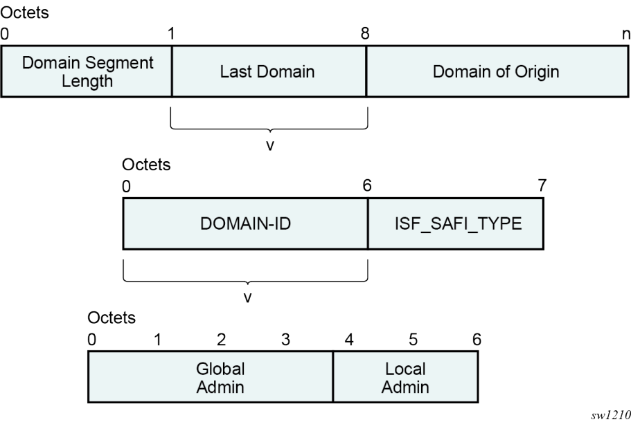
Figure 132: D-PATH attribute
