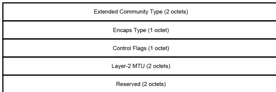
Figure 51: Layer 2 Info Extended Community attribute
