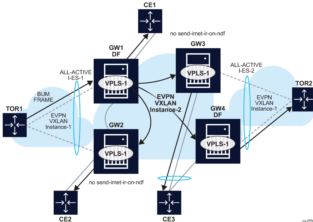
Figure 113: I-ES in dual EVPN-VXLAN services
