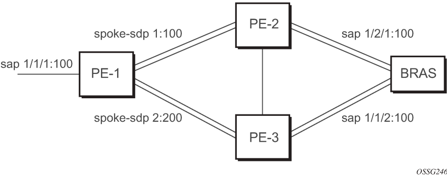
Figure 23: VLL resilience
