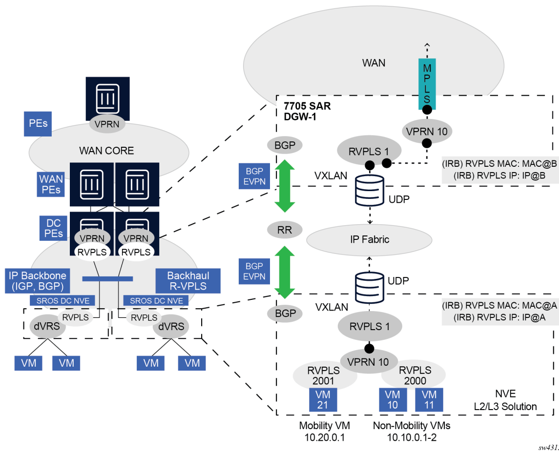
Figure 73: Gateway IRB on the DC PE for an L3 EVPN/VXLAN DC
