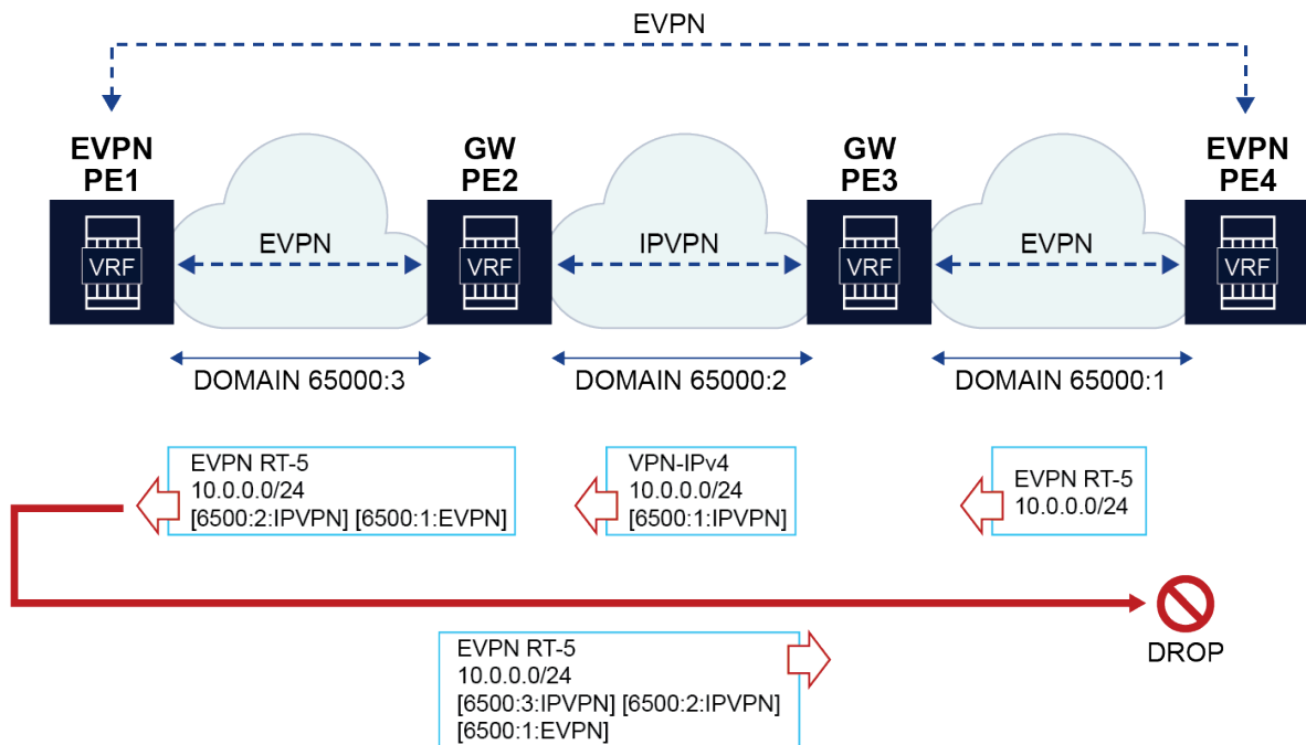
Figure 133: D-PATH attribute example
