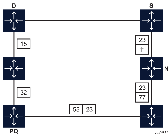
Figure 30: General principles of LDP rLFA operation
