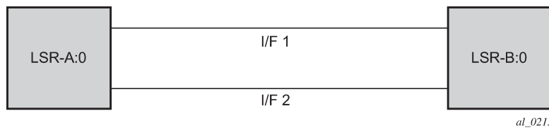
Figure 24: LDP adjacency and session over unnumbered interface
