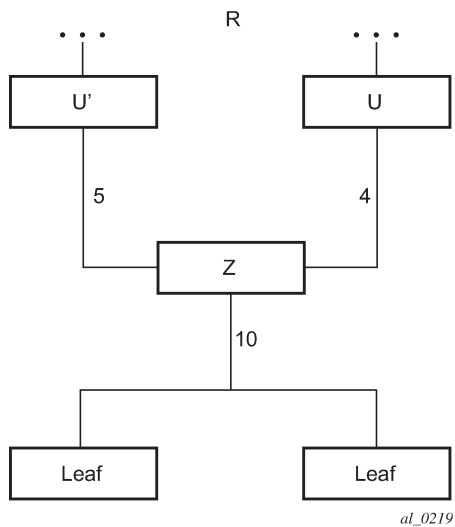
Figure 60: mLDP LSP with backup upstream LSR nodes
