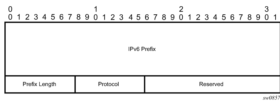
Figure 16: IPv6 IGP-prefix segment ID
