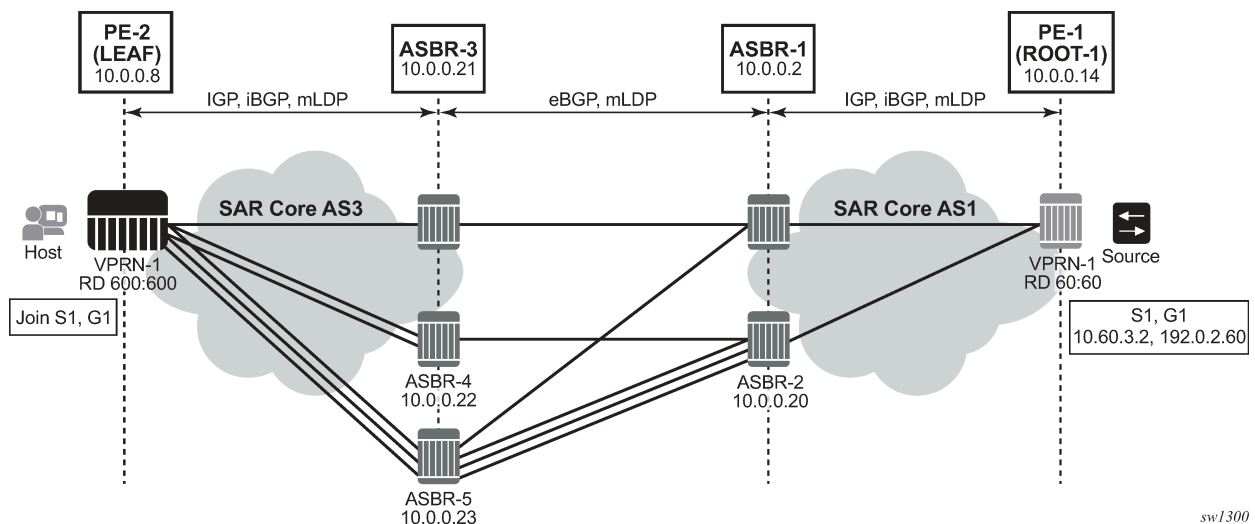
Figure 30: ECMP Support
