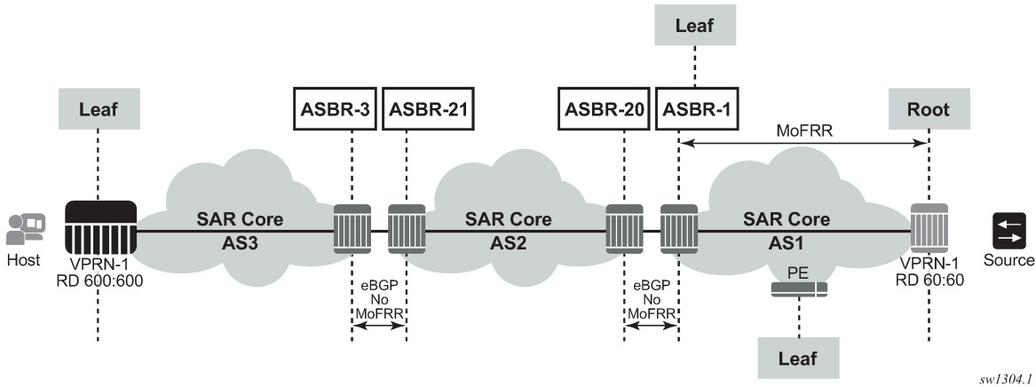
Figure 28: ASBRs Using EBGP Without IGP
