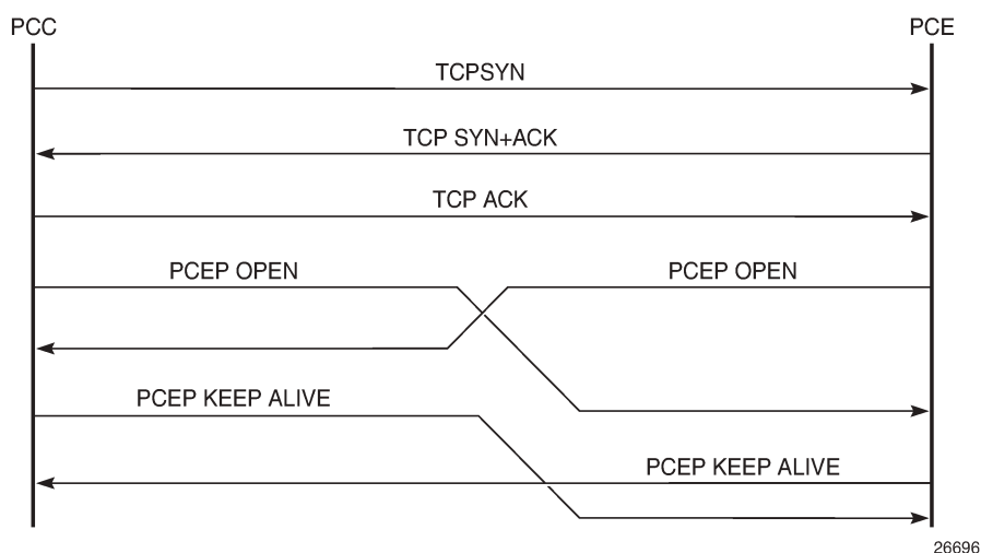
Figure 19: PCEP Session Initialization
