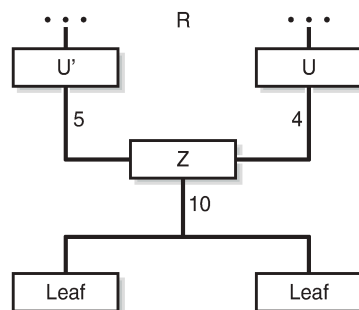
Figure 32: Multicast LDP Fast Upstream Switchover
