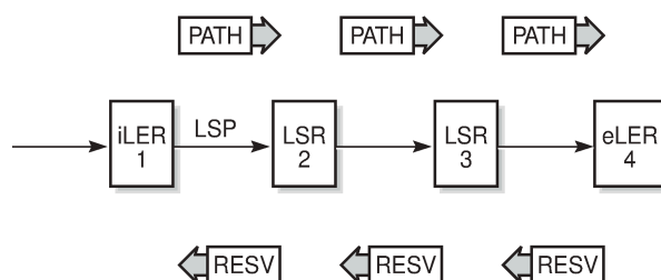
Figure 5: LSP Using RSVP-TE Path Setup displays an example of an LSP path set up using RSVP-TE. The ingress label edge router (iLER 1) transmits an RSVP-TE PATH message (path: 30.30.30.1)
