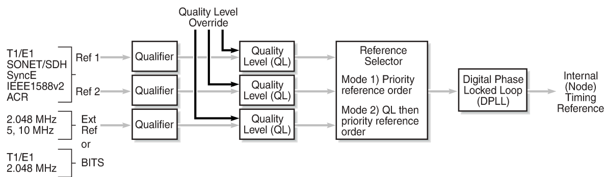
Figure 23: Timing reference selection based on quality level
