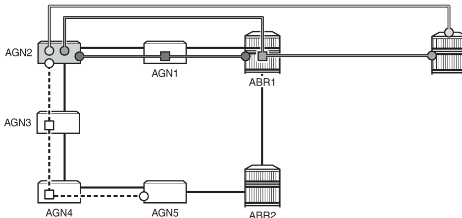
Figure 15: Label stack for remote LFA in ring topology
