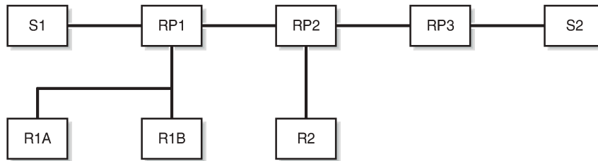
Figure 2: Anycast RP for PIM-SM implementation
