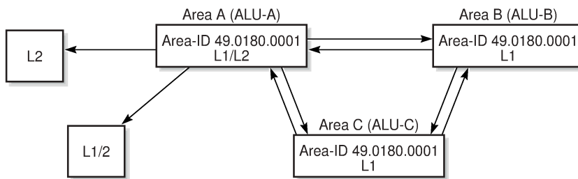
Figure 37: Configuring a level 1/2 area
