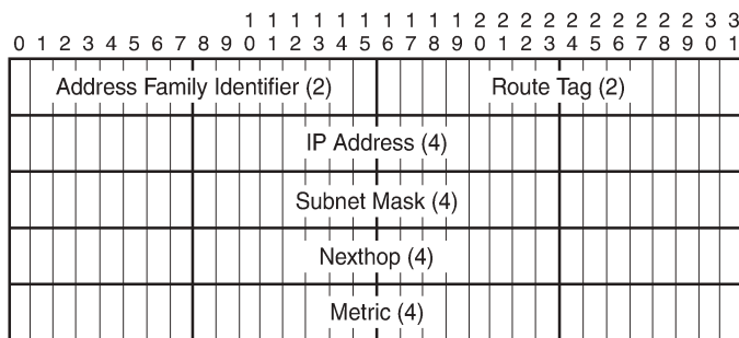
Figure 49: RIPv2 packet format
