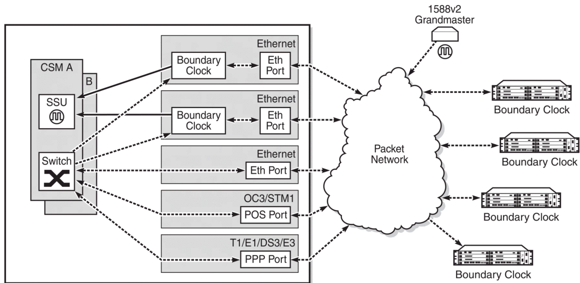
Figure 25: Boundary clock operation
