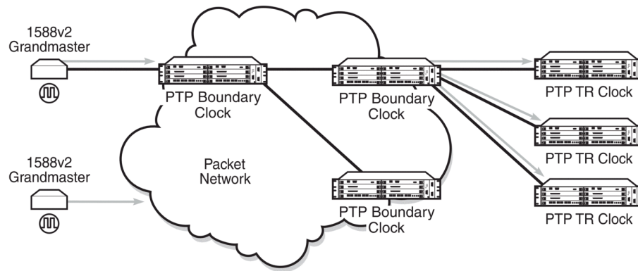
Figure 24: Boundary clock
