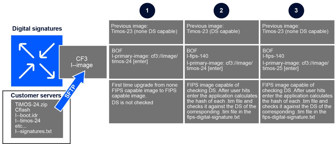
Figure 8: 7705 SAR DS environment
