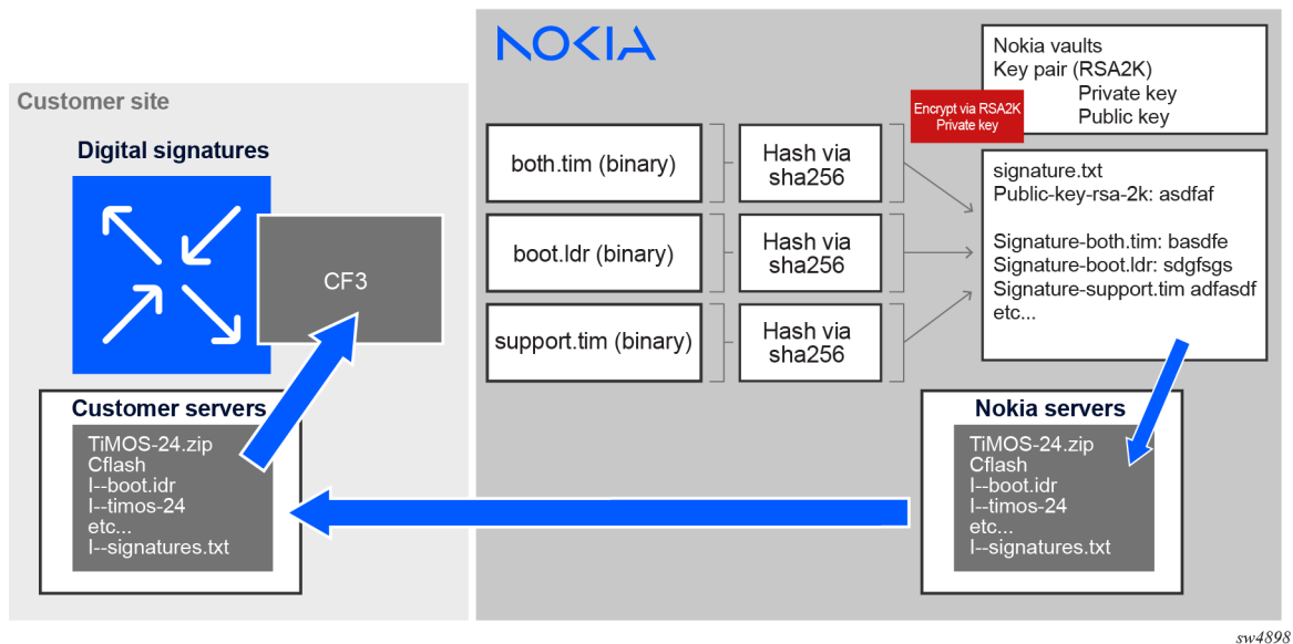
Figure 9: DS verification components
