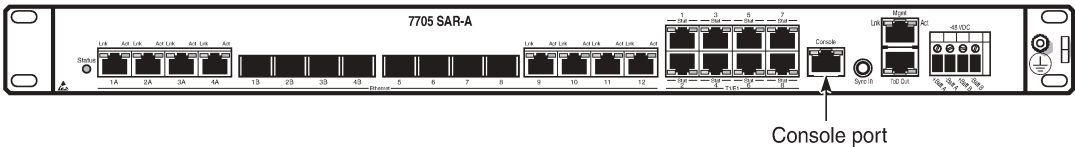
Figure 11: 7705 SAR Console port
