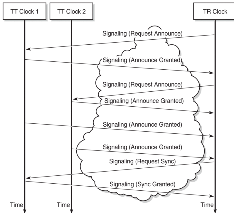
Figure 17: Messaging sequence between the PTP timeReceiver clock and PTP timeTransmitter clocks
