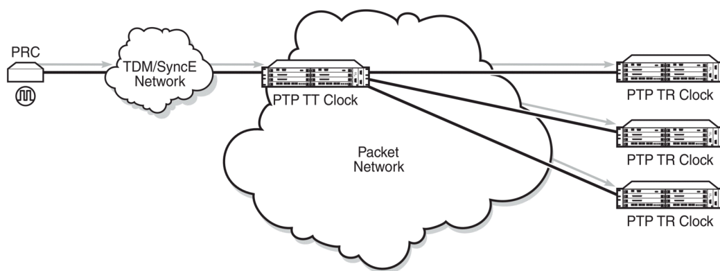
Figure 22: PTP timeTransmitter clock
