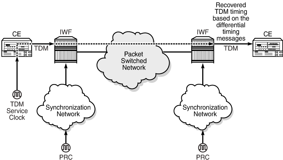
Figure 15: Differential clock recovery on a network
