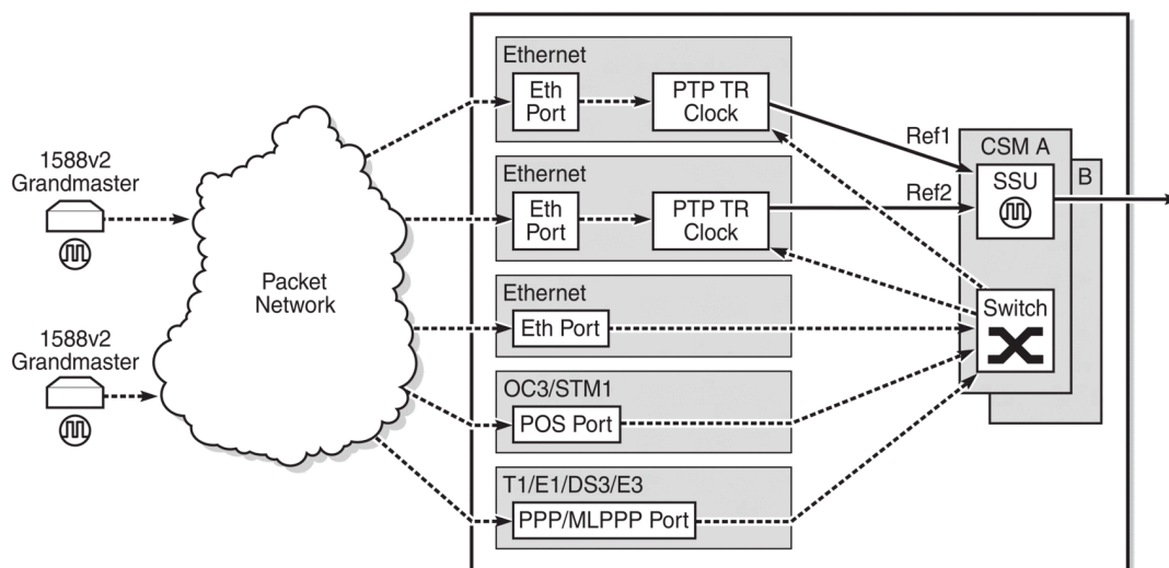
Figure 21: Ordinary timeReceiver clock operation
