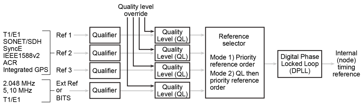
Figure 26: Timing reference selection based on quality level
