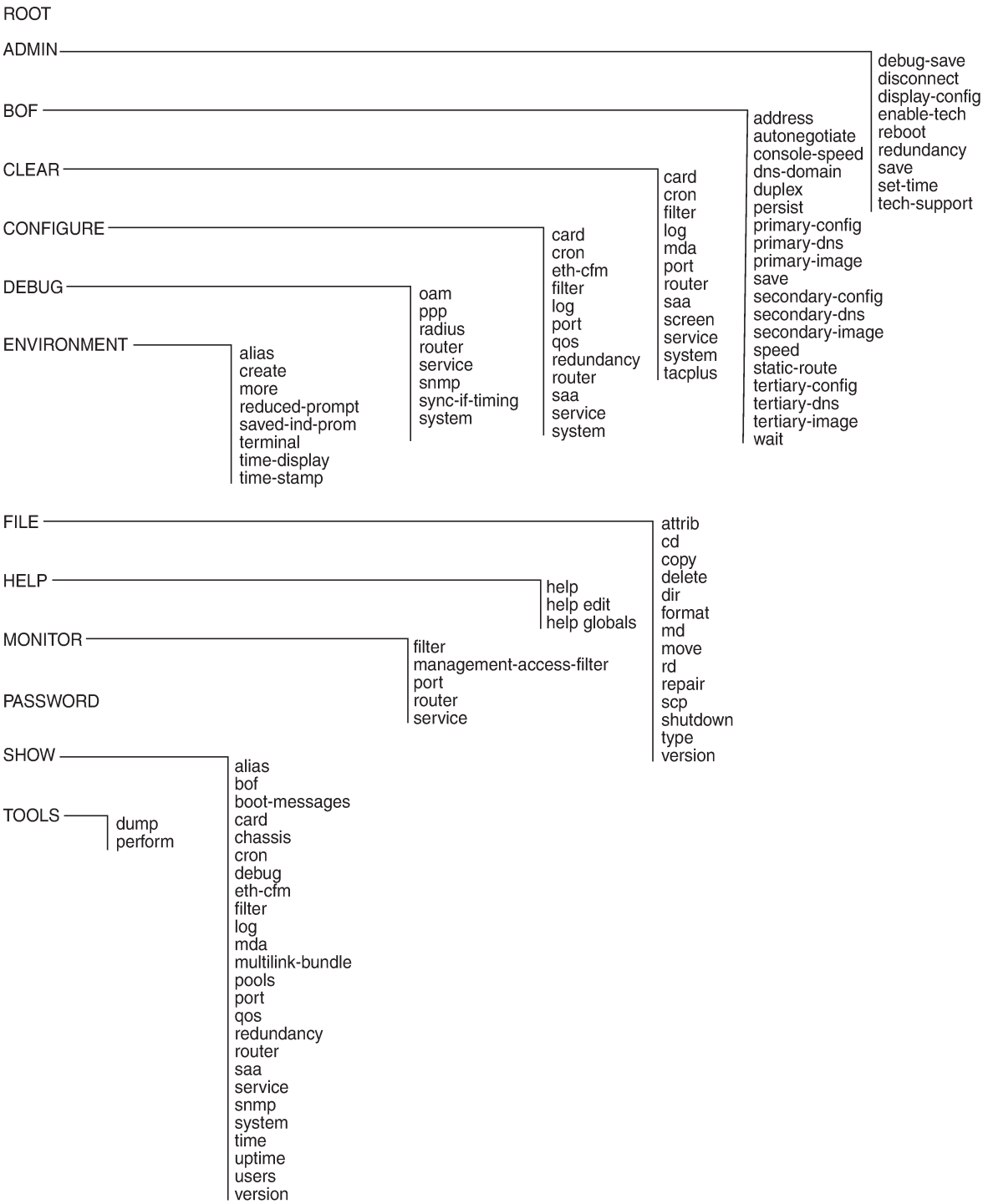
Figure 1: Root-level commands
