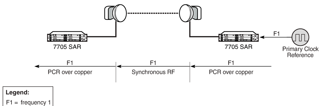
Figure 16: Proprietary clock recovery
