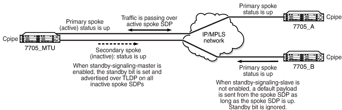
Figure 75: Standby-signaling-master enabled
