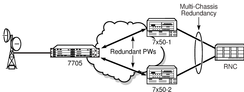
Figure 69: Pseudowire redundancy
