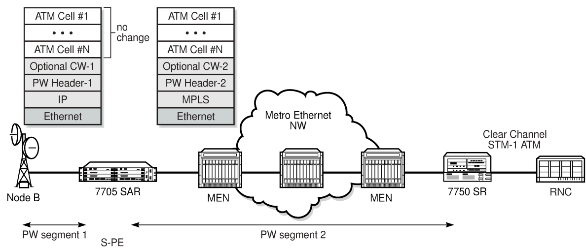
Figure 62: Simplex to simplex pseudowire switching
