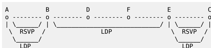
Testing LDP FEC of Node C with DSMAP TLV
