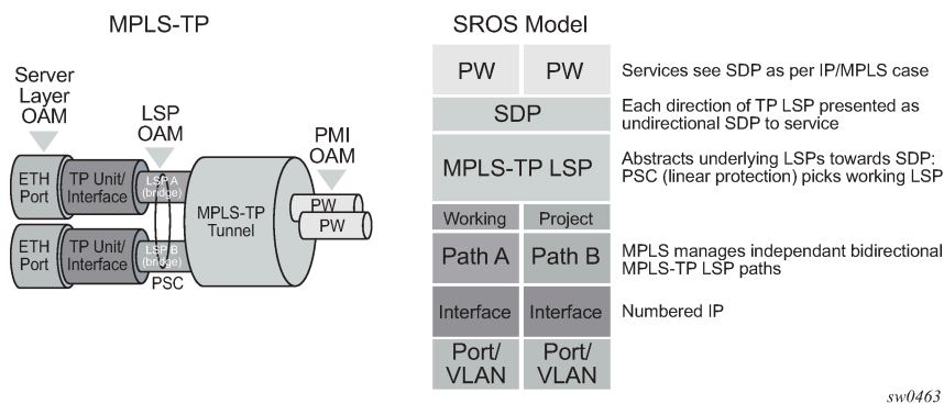
Figure 5: MPLS-TP model
