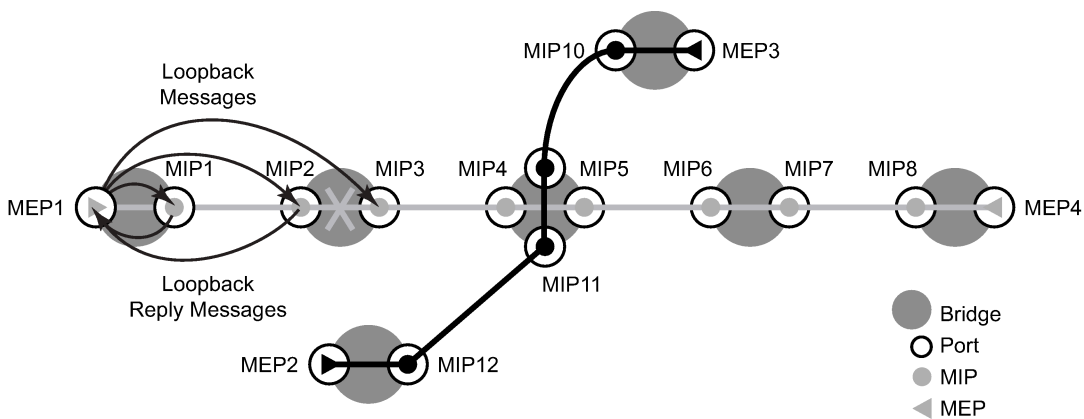
Figure 20: CFM loopback
